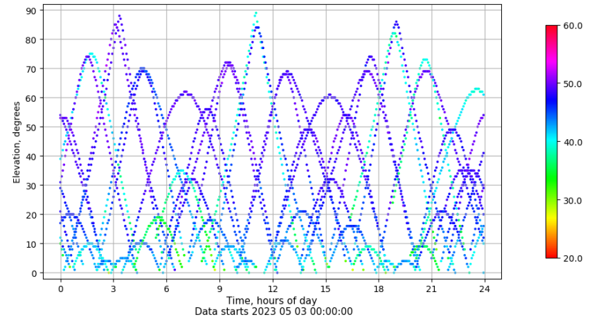
Time-elevation plot for station CANT. Signal to Noise S1C Data file CANT00ESP_R_2023123.xtr
