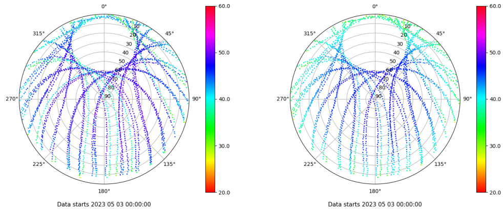
Skyplot for station CANT. Signal to Noise S1C Data file CANT00ESP_R_2023123.xtr Skyplot for station CANT. Signal to Noise S2P Data file CANT00ESP_R_2023123.xtr
