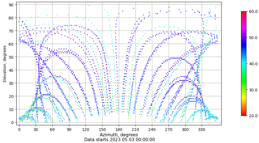
Azimuth-elevation plot for station CANT. Signal to Noise S1C Data file CANT00ESP_R_2023123.xtr
