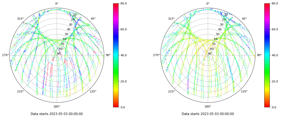
Skyplot for station CANT. Parameter M1C Data file CANT00ESP_R_2023123.xtr Skyplot for station CANT. Parameter M2P Data file CANT00ESP_R_2023123.xtr
