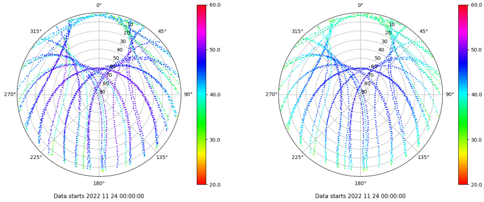
Skyplot for station CANT. Signal to Noise S1C Data file CANT00ESP_R_2022328.xtr Skyplot for station CANT. Signal to Noise S2P Data file CANT00ESP_R_2022328.xtr
