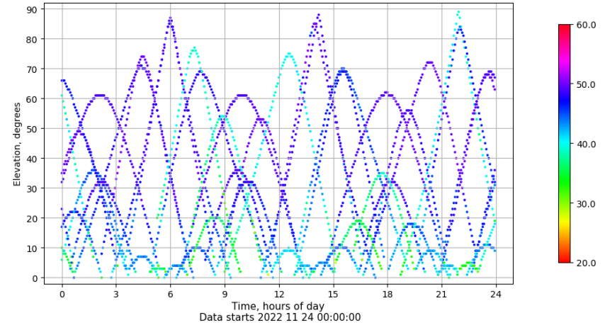
Time-elevation plot for station CANT. Signal to Noise S1C Data file CANT00ESP_R_2022328.xtr
