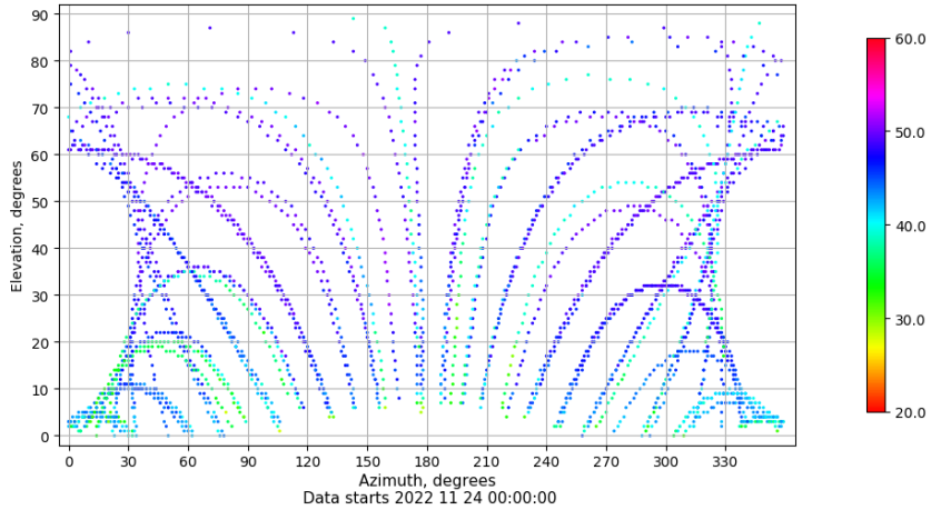
Azimuth-elevation plot for station CANT. Signal to Noise S1C Data file CANT00ESP_R_2022328.xtr
