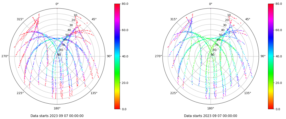
Skyplot for station CACE. Parameter M1C Data file CACE00ESP_R_2023250.xtr Skyplot for station CACE. Parameter M2C Data file CACE00ESP_R_2023250.xtr
