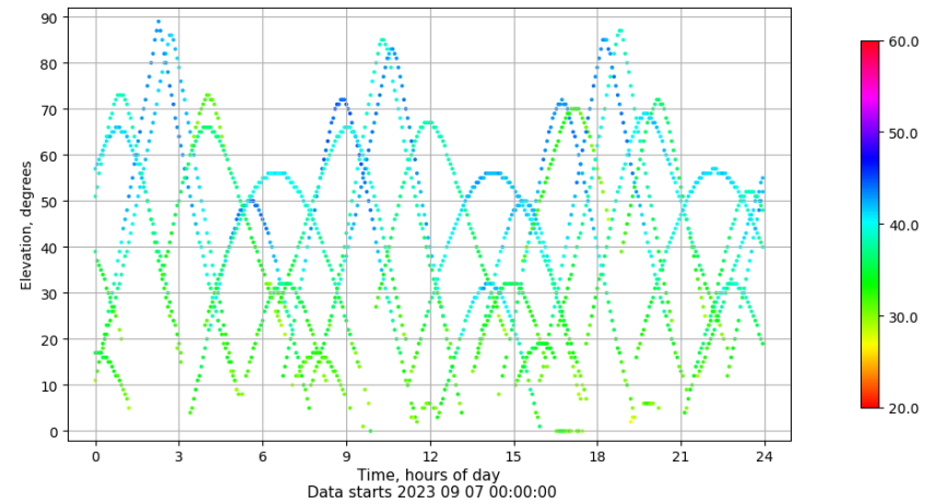
Time-elevation plot for station CACE. Signal to Noise S1C Data file CACE00ESP_R_2023250.xtr
