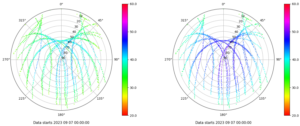
Skyplot for station CACE. Signal to Noise S1C Data file CACE00ESP_R_2023250.xtr Skyplot for station CACE. Signal to Noise S2C Data file CACE00ESP_R_2023250.xtr
