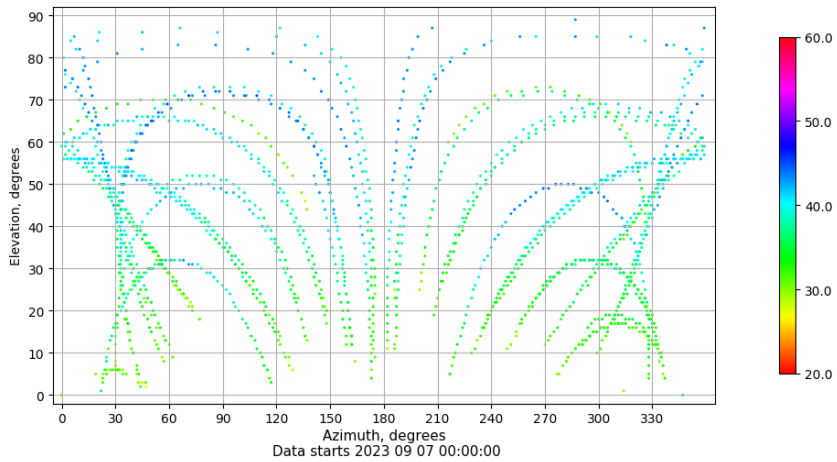
Azimuth-elevation plot for station CACE. Signal to Noise S1C Data file CACE00ESP_R_2023250.xtr
