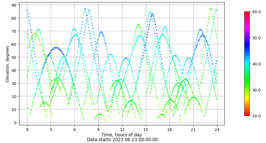
Time-elevation plot for station CACE. Signal to Noise S1C Data file CACE00ESP_R_2023174.xtr
