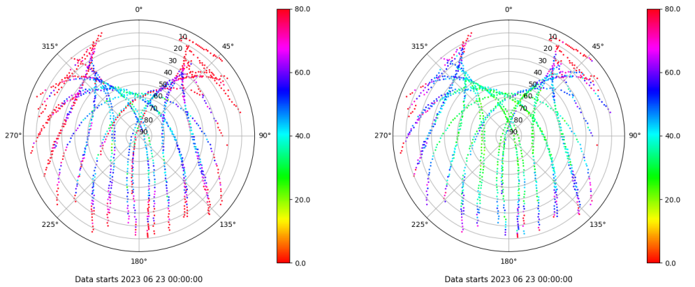
Skyplot for station CACE. Parameter M1C Data file CACE00ESP_R_2023174.xtr Skyplot for station CACE. Parameter M2C Data file CACE00ESP_R_2023174.xtr
