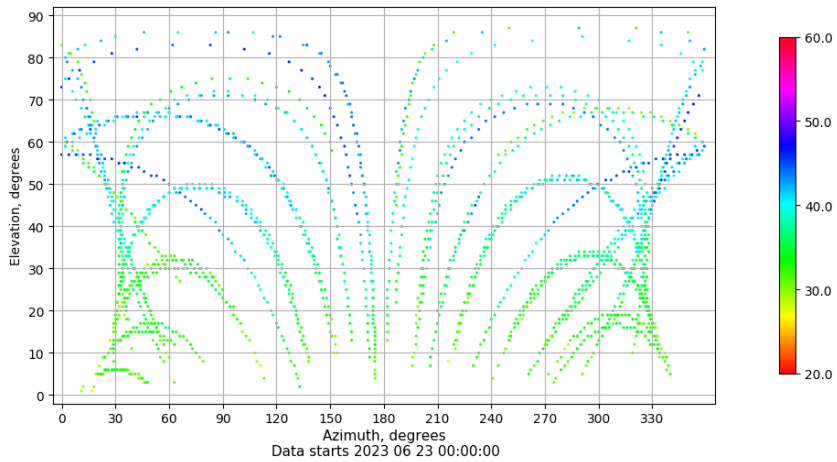
Azimuth-elevation plot for station CACE. Signal to Noise S1C Data file CACE00ESP_R_2023174.xtr
