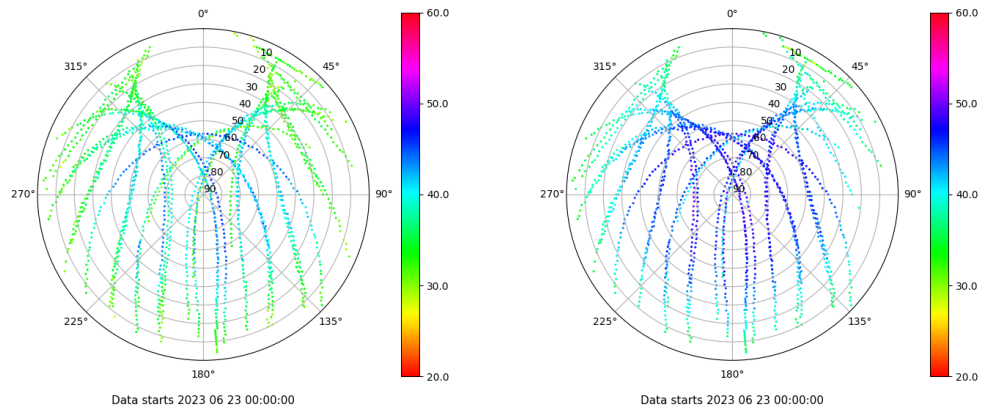
Skyplot for station CACE. Signal to Noise S1C Data file CACE00ESP_R_2023174.xtr Skyplot for station CACE. Signal to Noise S2C Data file CACE00ESP_R_2023174.xtr
