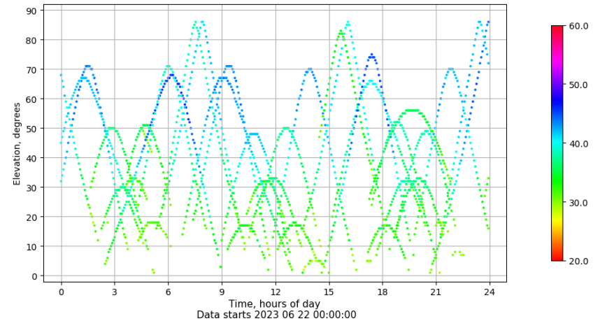
Time-elevation plot for station CACE. Signal to Noise S1C Data file CACE00ESP_R_2023173.xtr
