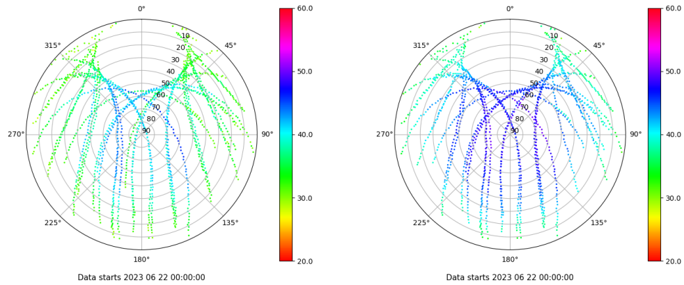
Skyplot for station CACE. Signal to Noise S1C Data file CACE00ESP_R_2023173.xtr Skyplot for station CACE. Signal to Noise S2C Data file CACE00ESP_R_2023173.xtr
