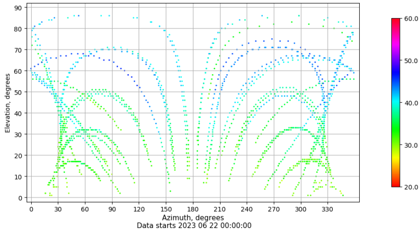
Azimuth-elevation plot for station CACE. Signal to Noise S1C Data file CACE00ESP_R_2023173.xtr
