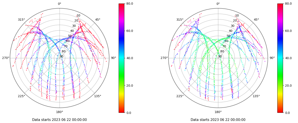
Skyplot for station CACE. Parameter M1C Data file CACE00ESP_R_2023173.xtr Skyplot for station CACE. Parameter M2C Data file CACE00ESP_R_2023173.xtr
