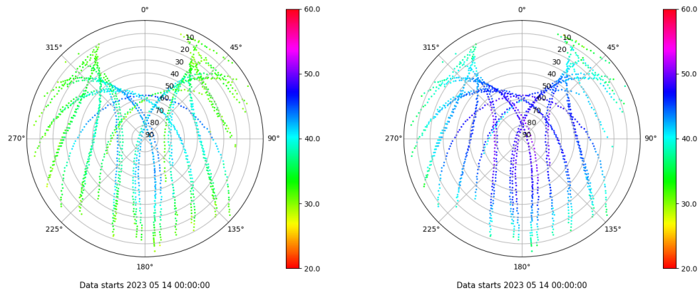
Skyplot for station CACE. Signal to Noise S1C Data file CACE00ESP_R_2023134.xtr Skyplot for station CACE. Signal to Noise S2C Data file CACE00ESP_R_2023134.xtr
