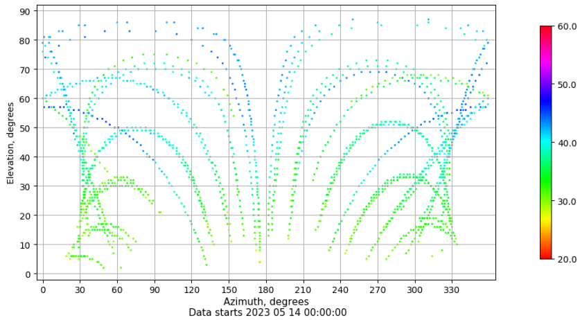
Azimuth-elevation plot for station CACE. Signal to Noise S1C Data file CACE00ESP_R_2023134.xtr
