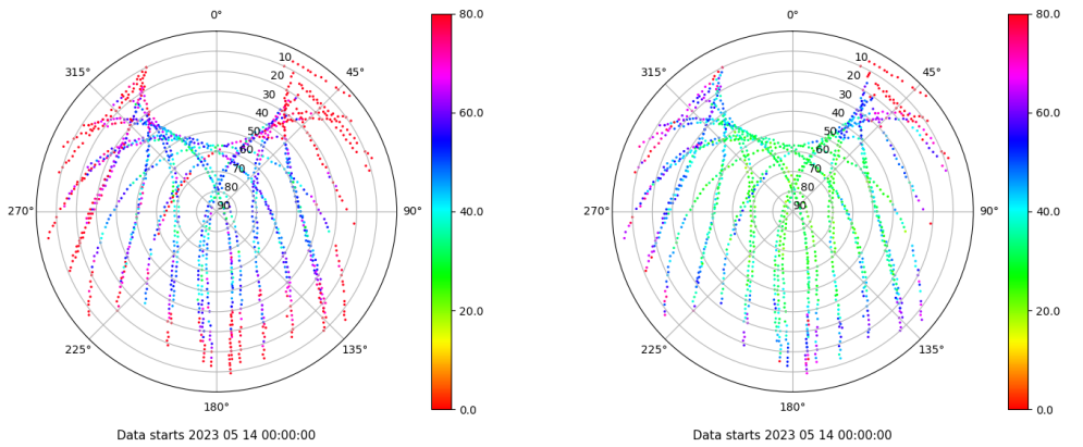
Skyplot for station CACE. Parameter M1C Data file CACE00ESP_R_2023134.xtr Skyplot for station CACE. Parameter M2C Data file CACE00ESP_R_2023134.xtr
