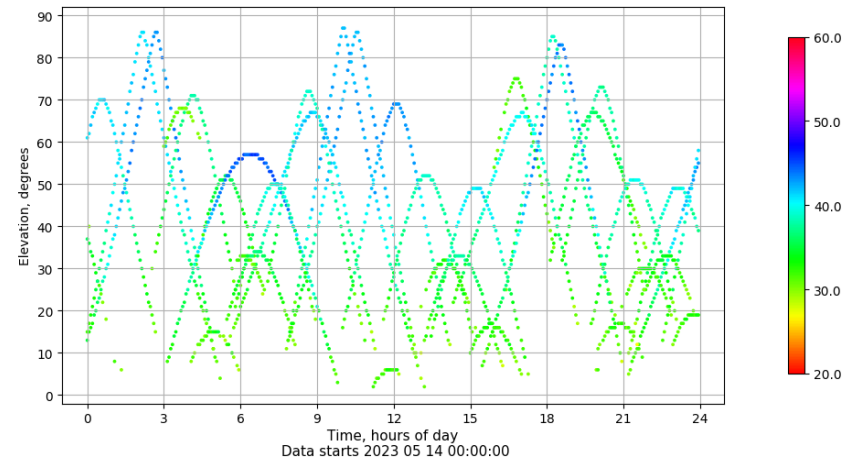
Time-elevation plot for station CACE. Signal to Noise S1C Data file CACE00ESP_R_2023134.xtr
