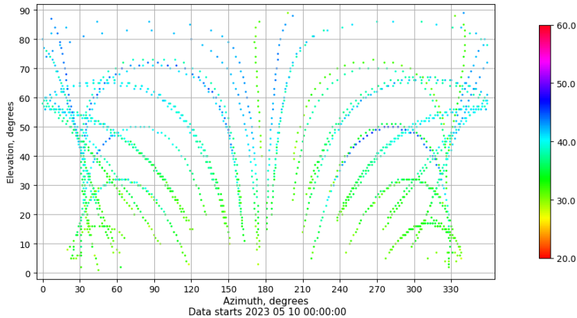
Azimuth-elevation plot for station CACE. Signal to Noise S1C Data file CACE00ESP_R_2023130.xtr
