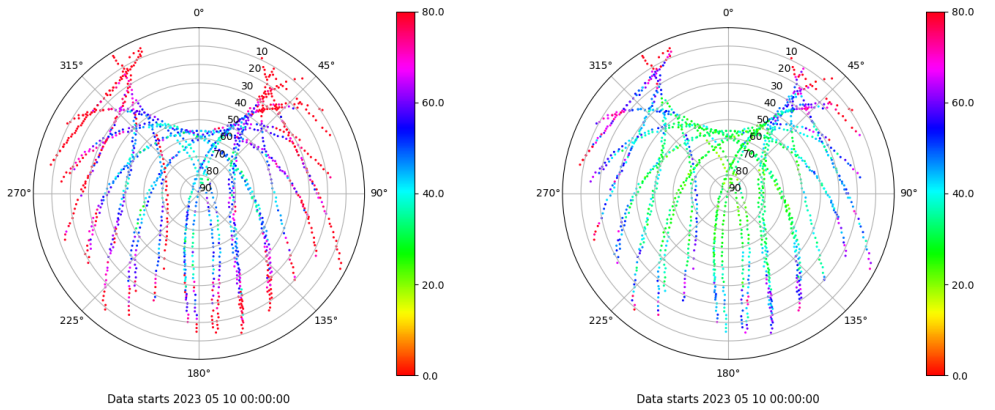
Skyplot for station CACE. Parameter M1C Data file CACE00ESP_R_2023130.xtr Skyplot for station CACE. Parameter M2C Data file CACE00ESP_R_2023130.xtr
