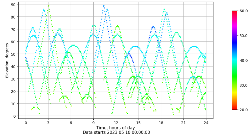
Time-elevation plot for station CACE. Signal to Noise S1C Data file CACE00ESP_R_2023130.xtr
