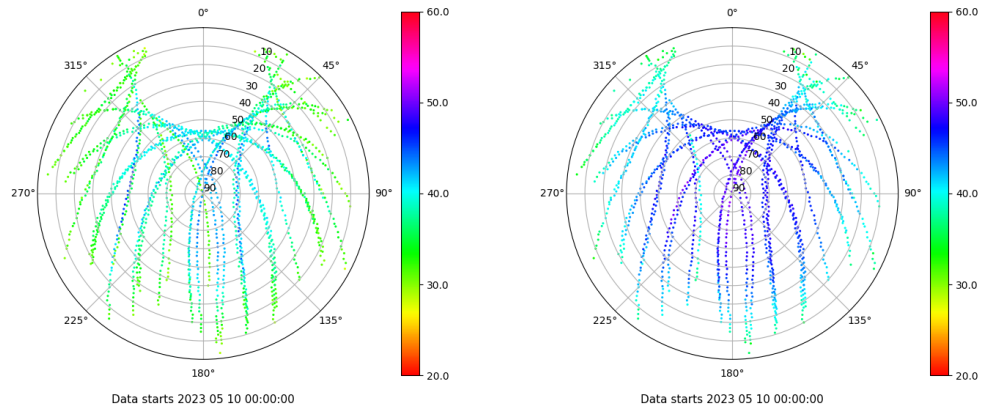
Skyplot for station CACE. Signal to Noise S1C Data file CACE00ESP_R_2023130.xtr Skyplot for station CACE. Signal to Noise S2C Data file CACE00ESP_R_2023130.xtr
