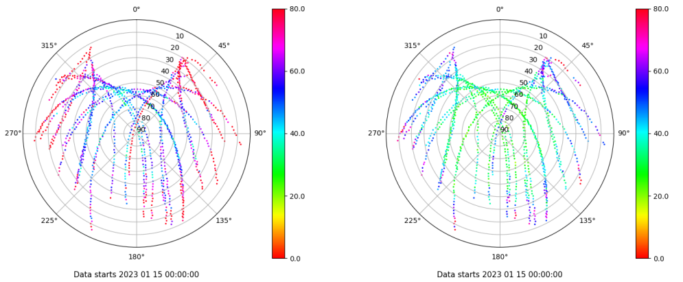
Skyplot for station CACE. Parameter M1C Data file CACE00ESP_R_2023015.xtr Skyplot for station CACE. Parameter M2C Data file CACE00ESP_R_2023015.xtr
