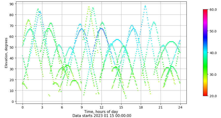
Time-elevation plot for station CACE. Signal to Noise S1C Data file CACE00ESP_R_2023015.xtr
