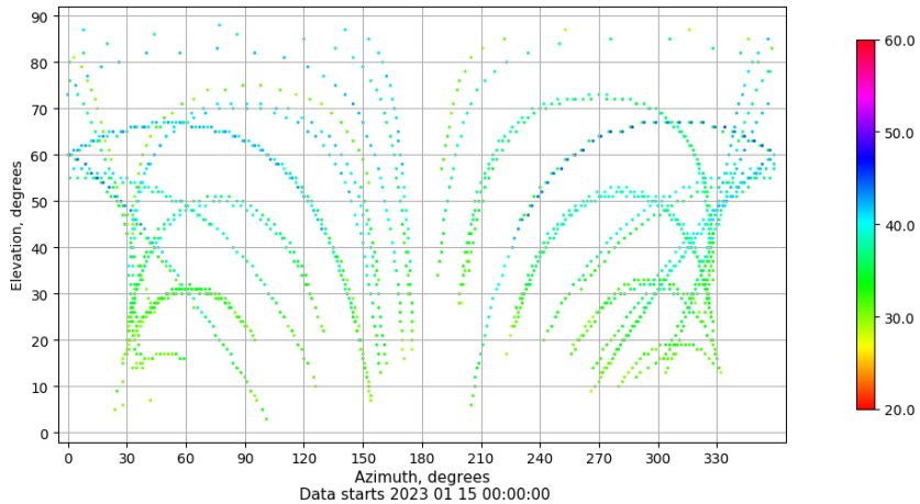
Azimuth-elevation plot for station CACE. Signal to Noise S1C Data file CACE00ESP_R_2023015.xtr
