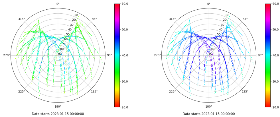
Skyplot for station CACE. Signal to Noise S1C Data file CACE00ESP_R_2023015.xtr Skyplot for station CACE. Signal to Noise S2C Data file CACE00ESP_R_2023015.xtr
