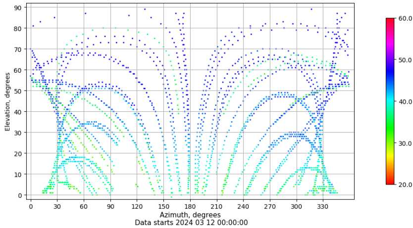
Azimuth-elevation plot for station CAAL. Signal to Noise S1C Data file CAAL00ESP_R_2024072.xtr
