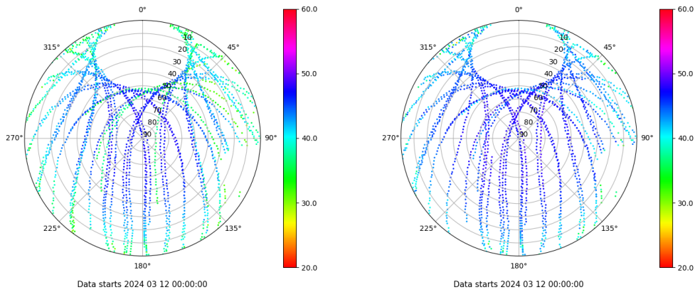
Skyplot for station CAAL. Signal to Noise S1C Data file CAAL00ESP_R_2024072.xtr Skyplot for station CAAL. Signal to Noise S2P Data file CAAL00ESP_R_2024072.xtr
