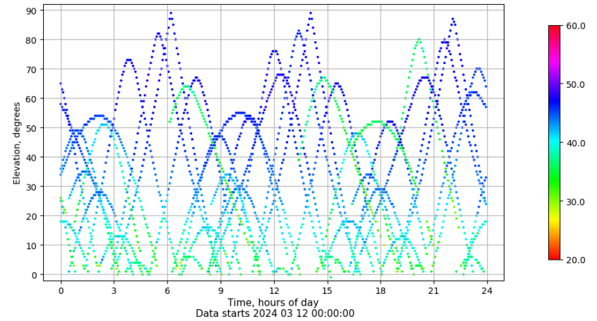
Time-elevation plot for station CAAL. Signal to Noise S1C Data file CAAL00ESP_R_2024072.xtr
