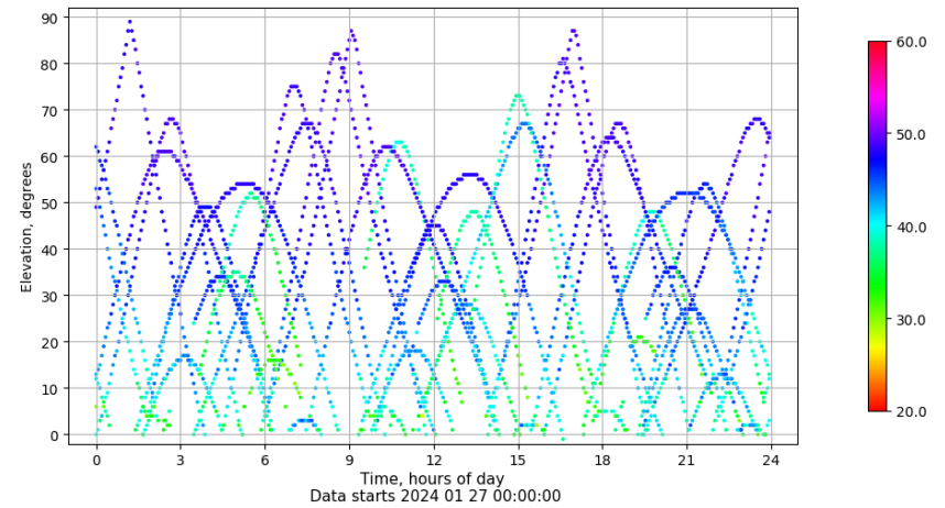
Time-elevation plot for station CAAL. Signal to Noise S1C Data file CAAL00ESP_R_2024027.xtr
