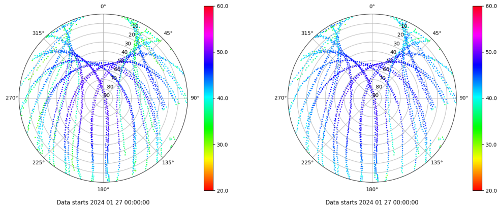
Skyplot for station CAAL. Signal to Noise S1C Data file CAAL00ESP_R_2024027.xtr Skyplot for station CAAL. Signal to Noise S2P Data file CAAL00ESP_R_2024027.xtr
