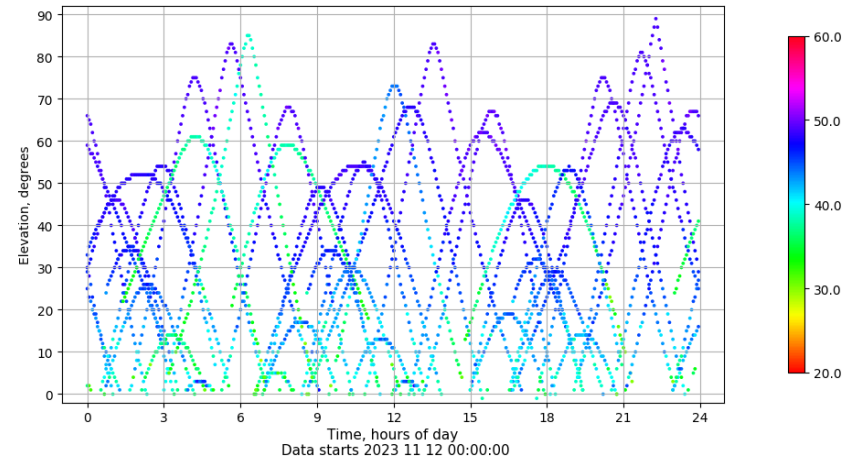
Time-elevation plot for station CAAL. Signal to Noise S1C Data file CAAL00ESP_R_2023316.xtr
