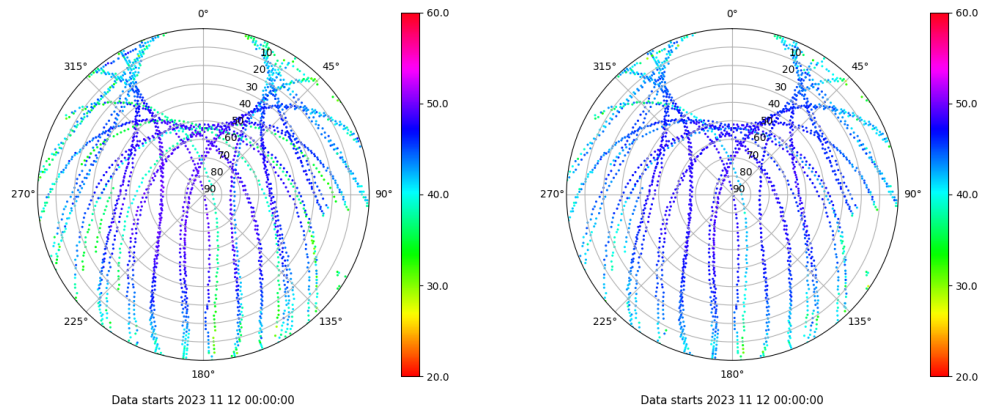
Skyplot for station CAAL. Signal to Noise S1C Data file CAAL00ESP_R_2023316.xtr Skyplot for station CAAL. Signal to Noise S2P Data file CAAL00ESP_R_2023316.xtr
