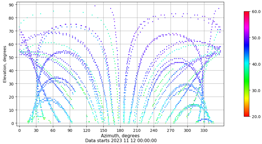
Azimuth-elevation plot for station CAAL. Signal to Noise S1C Data file CAAL00ESP_R_2023316.xtr
