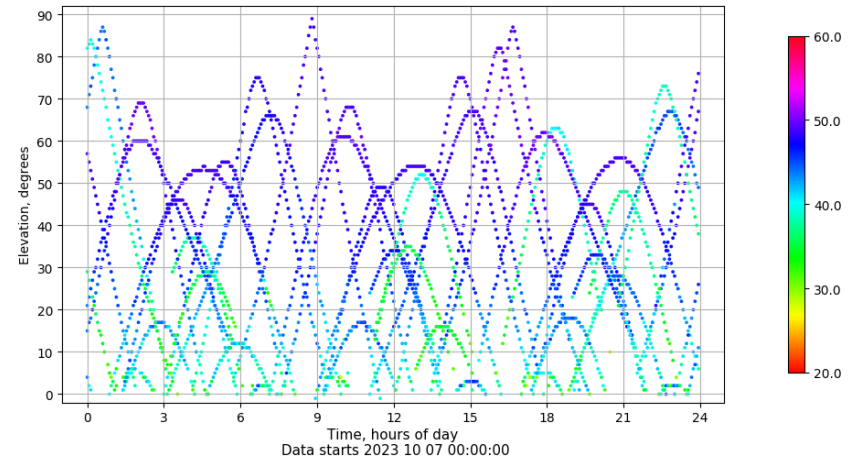
Time-elevation plot for station CAAL. Signal to Noise S1C Data file CAAL00ESP_R_2023280.xtr
