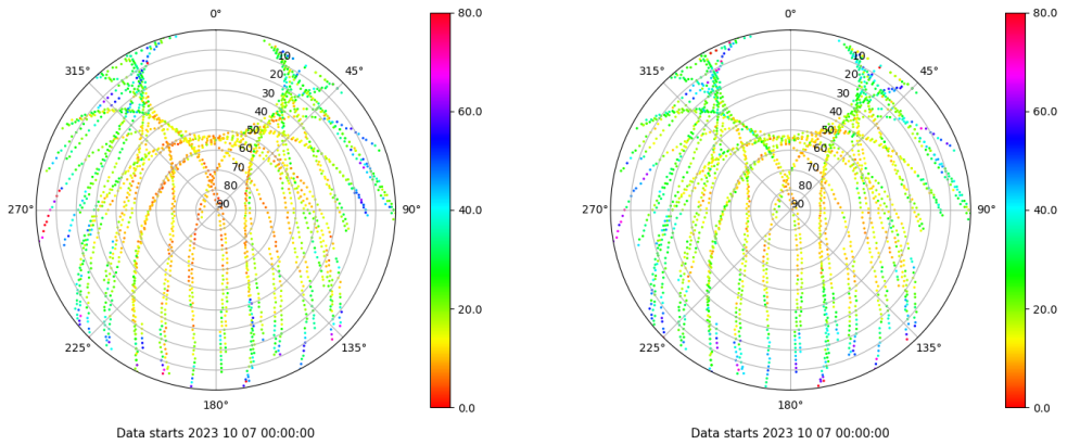
Skyplot for station CAAL. Parameter M1C Data file CAAL00ESP_R_2023280.xtr Skyplot for station CAAL. Parameter M2P Data file CAAL00ESP_R_2023280.xtr
