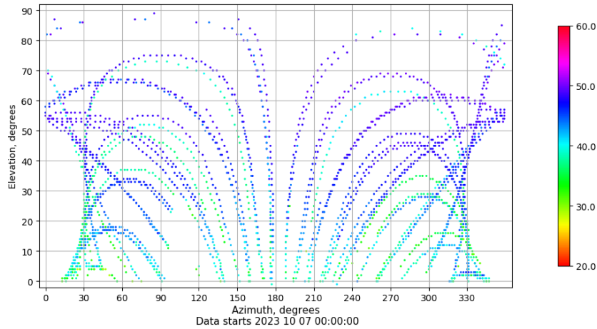
Azimuth-elevation plot for station CAAL. Signal to Noise S1C Data file CAAL00ESP_R_2023280.xtr
