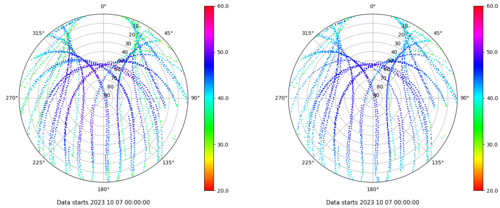
Skyplot for station CAAL. Signal to Noise S1C Data file CAAL00ESP_R_2023280.xtr Skyplot for station CAAL. Signal to Noise S2P Data file CAAL00ESP_R_2023280.xtr
