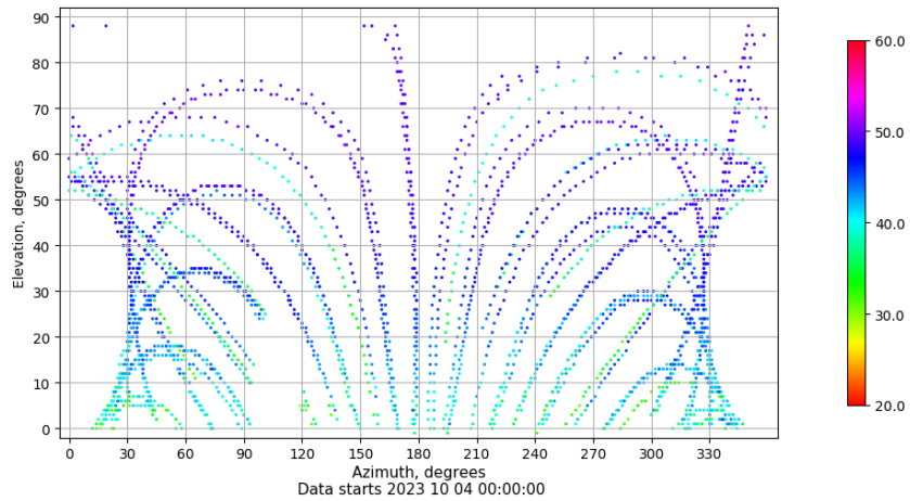
Azimuth-elevation plot for station CAAL. Signal to Noise S1C Data file CAAL00ESP_R_2023277.xtr
