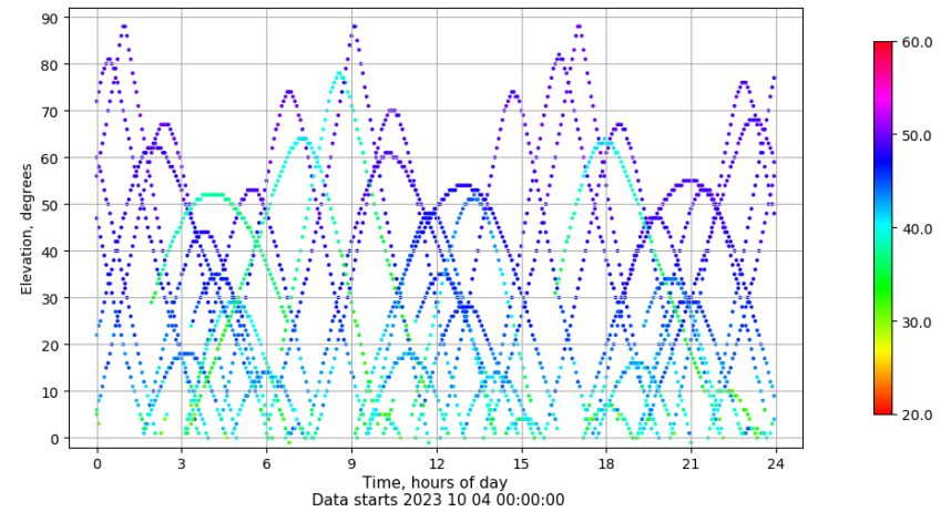
Time-elevation plot for station CAAL. Signal to Noise S1C Data file CAAL00ESP_R_2023277.xtr
