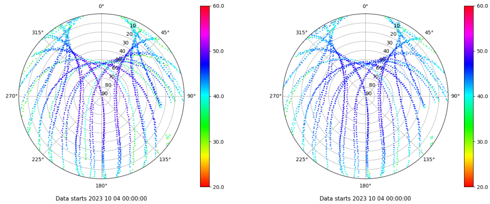
Skyplot for station CAAL. Signal to Noise S1C Data file CAAL00ESP_R_2023277.xtr Skyplot for station CAAL. Signal to Noise S2P Data file CAAL00ESP_R_2023277.xtr
