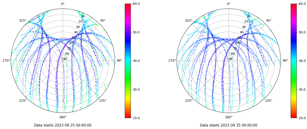
Skyplot for station CAAL. Signal to Noise S1C Data file CAAL00ESP_R_2023268.xtr Skyplot for station CAAL. Signal to Noise S2P Data file CAAL00ESP_R_2023268.xtr
