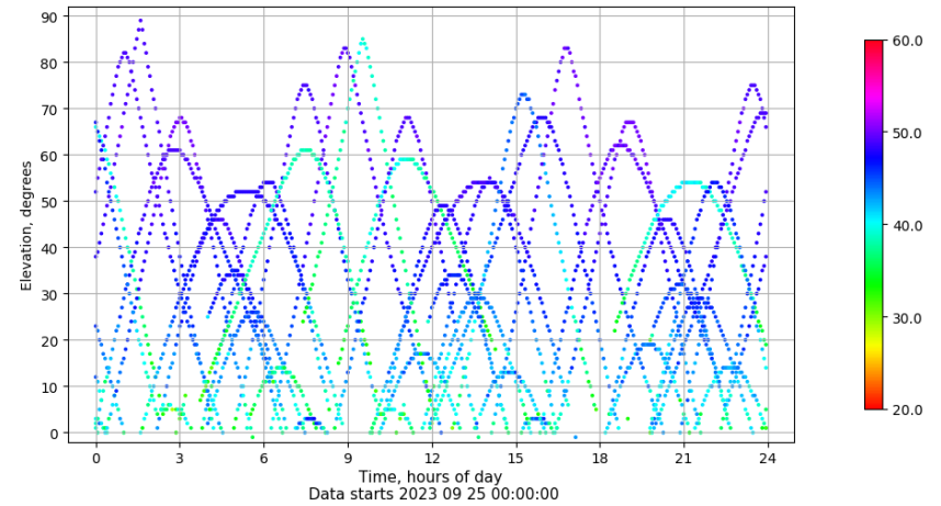
Time-elevation plot for station CAAL. Signal to Noise S1C Data file CAAL00ESP_R_2023268.xtr
