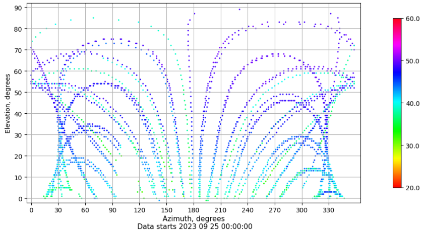
Azimuth-elevation plot for station CAAL. Signal to Noise S1C Data file CAAL00ESP_R_2023268.xtr
