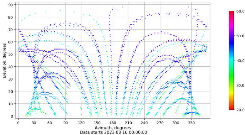
Azimuth-elevation plot for station CAAL. Signal to Noise S1C Data file CAAL00ESP_R_2023228.xtr
