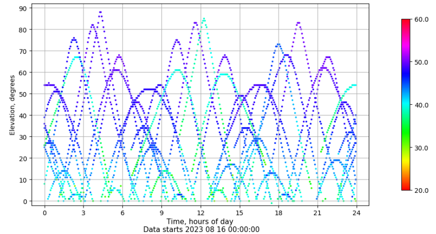
Time-elevation plot for station CAAL. Signal to Noise S1C Data file CAAL00ESP_R_2023228.xtr
