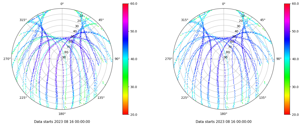
Skyplot for station CAAL. Signal to Noise S1C Data file CAAL00ESP_R_2023228.xtr Skyplot for station CAAL. Signal to Noise S2P Data file CAAL00ESP_R_2023228.xtr
