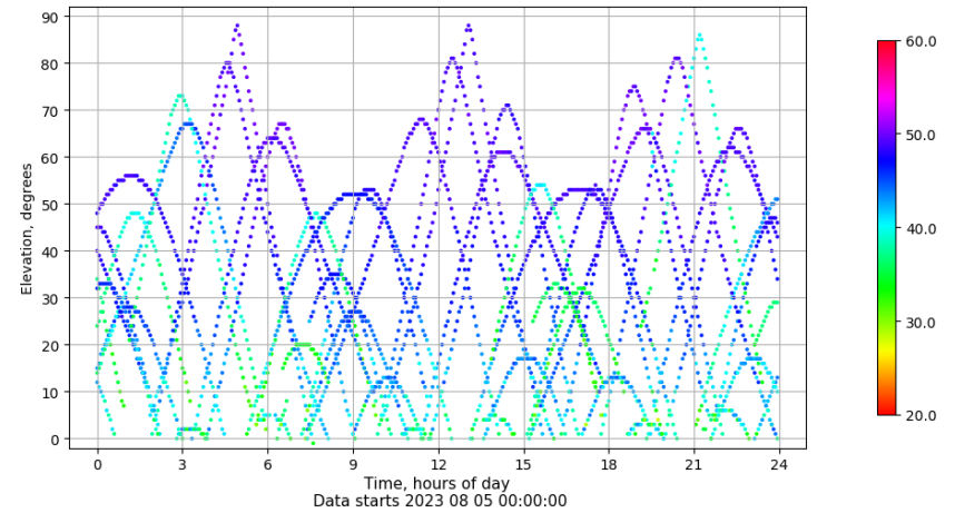
Time-elevation plot for station CAAL. Signal to Noise S1C Data file CAAL00ESP_R_2023217.xtr
