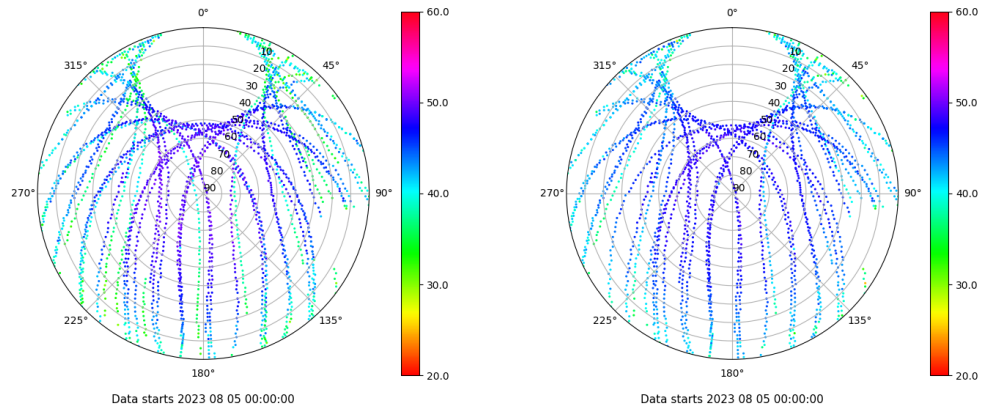
Skyplot for station CAAL. Signal to Noise S1C Data file CAAL00ESP_R_2023217.xtr Skyplot for station CAAL. Signal to Noise S2P Data file CAAL00ESP_R_2023217.xtr
