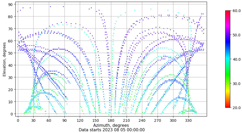
Azimuth-elevation plot for station CAAL. Signal to Noise S1C Data file CAAL00ESP_R_2023217.xtr
