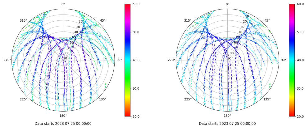
Skyplot for station CAAL. Signal to Noise S1C Data file CAAL00ESP_R_2023206.xtr Skyplot for station CAAL. Signal to Noise S2P Data file CAAL00ESP_R_2023206.xtr
