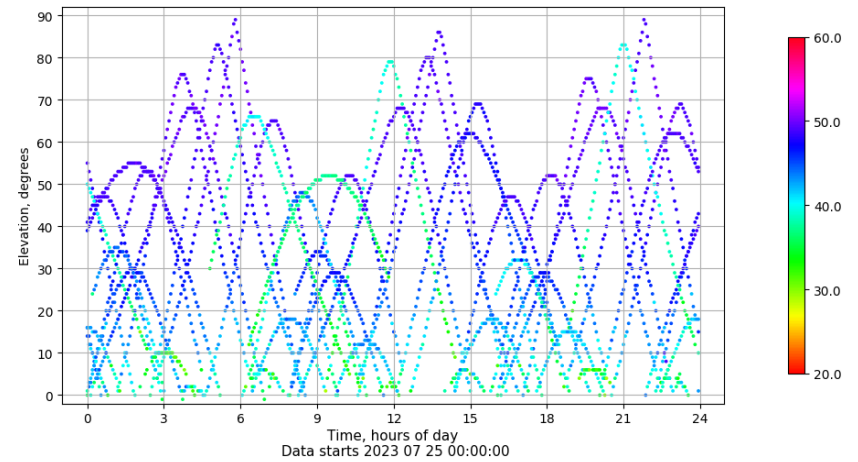
Time-elevation plot for station CAAL. Signal to Noise S1C Data file CAAL00ESP_R_2023206.xtr
