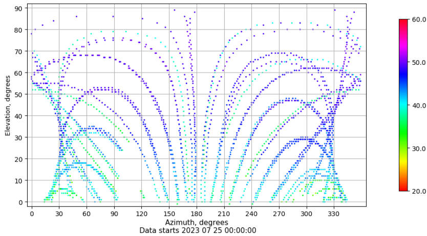
Azimuth-elevation plot for station CAAL. Signal to Noise S1C Data file CAAL00ESP_R_2023206.xtr
