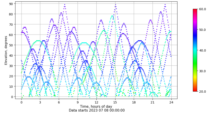
Time-elevation plot for station CAAL. Signal to Noise S1C Data file CAAL00ESP_R_2023189.xtr
