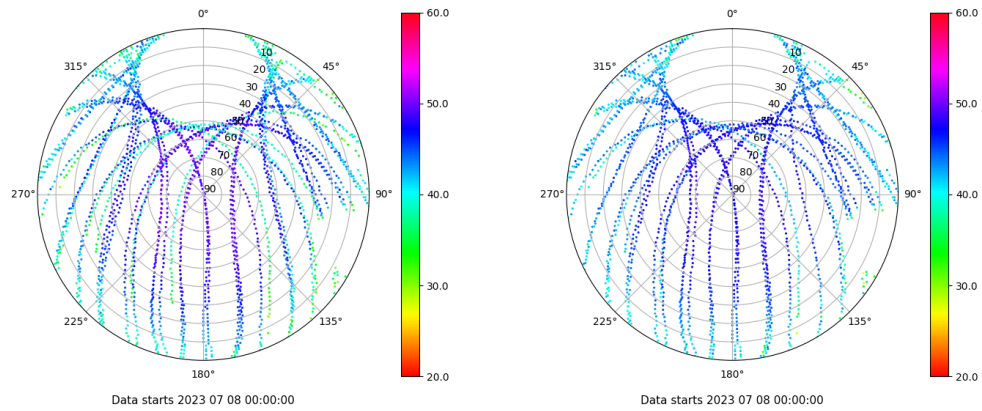
Skyplot for station CAAL. Signal to Noise S1C Data file CAAL00ESP_R_2023189.xtr Skyplot for station CAAL. Signal to Noise S2P Data file CAAL00ESP_R_2023189.xtr
