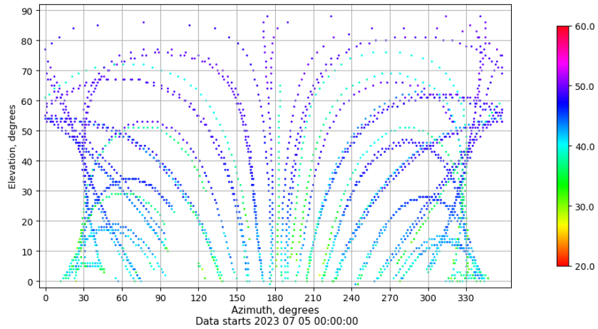
Azimuth-elevation plot for station CAAL. Signal to Noise S1C Data file CAAL00ESP_R_2023186.xtr
