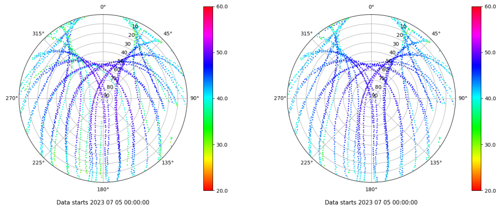
Skyplot for station CAAL. Signal to Noise S1C Data file CAAL00ESP_R_2023186.xtr Skyplot for station CAAL. Signal to Noise S2P Data file CAAL00ESP_R_2023186.xtr
