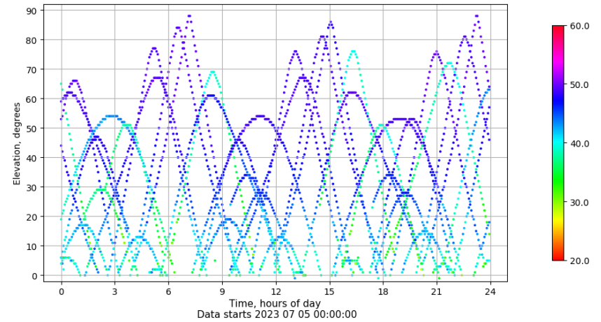
Time-elevation plot for station CAAL. Signal to Noise S1C Data file CAAL00ESP_R_2023186.xtr
