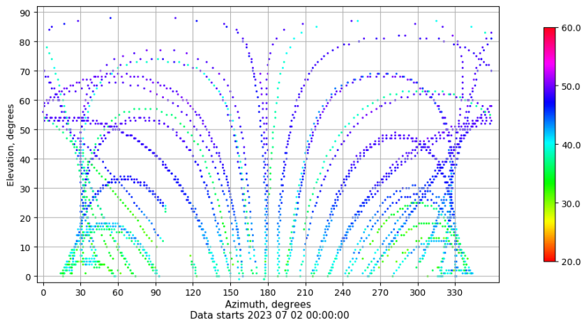
Azimuth-elevation plot for station CAAL. Signal to Noise S1C Data file CAAL00ESP_R_2023183.xtr
