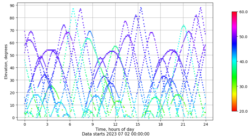
Time-elevation plot for station CAAL. Signal to Noise S1C Data file CAAL00ESP_R_2023183.xtr
