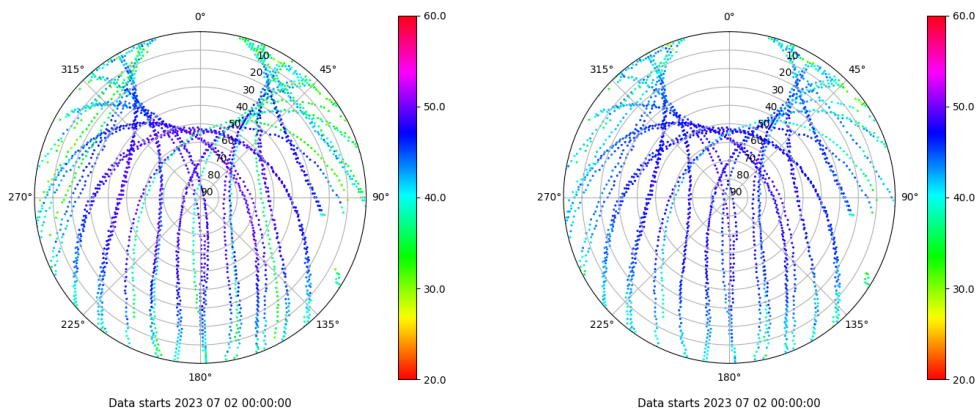
Skyplot for station CAAL. Signal to Noise S1C Data file CAAL00ESP_R_2023183.xtr Skyplot for station CAAL. Signal to Noise S2P Data file CAAL00ESP_R_2023183.xtr
