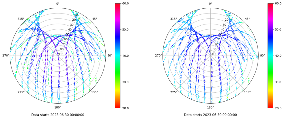
Skyplot for station CAAL. Signal to Noise S1C Data file CAAL00ESP_R_2023181.xtr Skyplot for station CAAL. Signal to Noise S2P Data file CAAL00ESP_R_2023181.xtr
