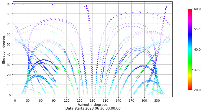
Azimuth-elevation plot for station CAAL. Signal to Noise S1C Data file CAAL00ESP_R_2023181.xtr
