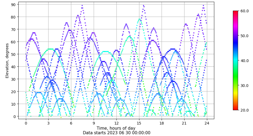
Time-elevation plot for station CAAL. Signal to Noise S1C Data file CAAL00ESP_R_2023181.xtr
