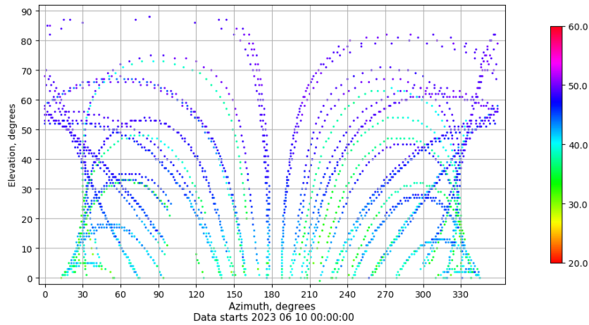
Azimuth-elevation plot for station CAAL. Signal to Noise S1C Data file CAAL00ESP_R_2023161.xtr
