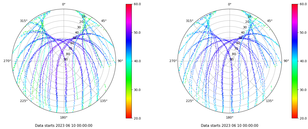
Skyplot for station CAAL. Signal to Noise S1C Data file CAAL00ESP_R_2023161.xtr Skyplot for station CAAL. Signal to Noise S2P Data file CAAL00ESP_R_2023161.xtr
