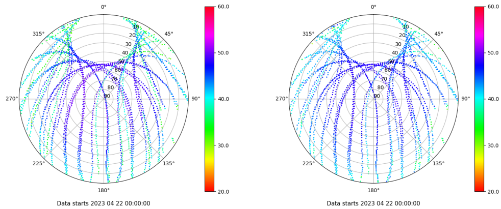
Skyplot for station CAAL. Signal to Noise S1C Data file CAAL00ESP_R_2023112.xtr Skyplot for station CAAL. Signal to Noise S2P Data file CAAL00ESP_R_2023112.xtr
