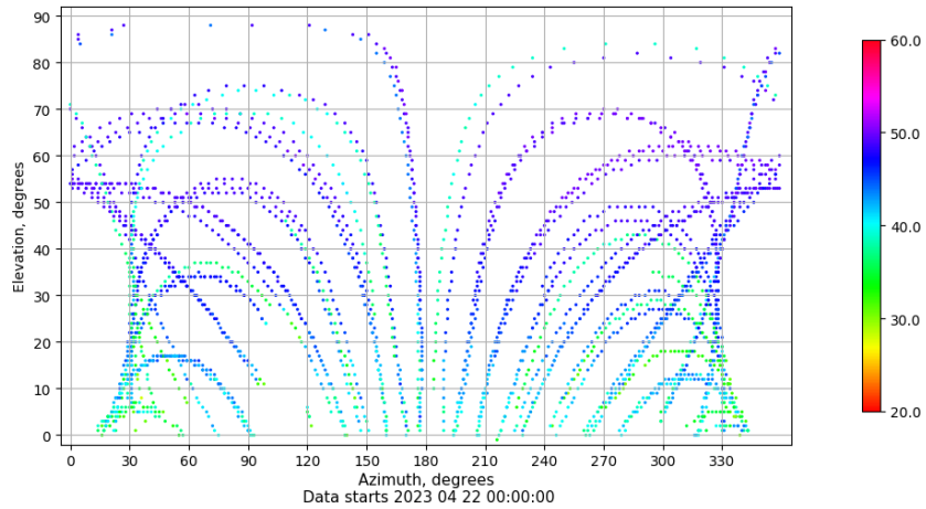
Azimuth-elevation plot for station CAAL. Signal to Noise S1C Data file CAAL00ESP_R_2023112.xtr
