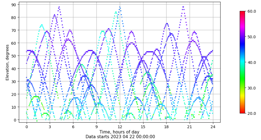
Time-elevation plot for station CAAL. Signal to Noise S1C Data file CAAL00ESP_R_2023112.xtr
