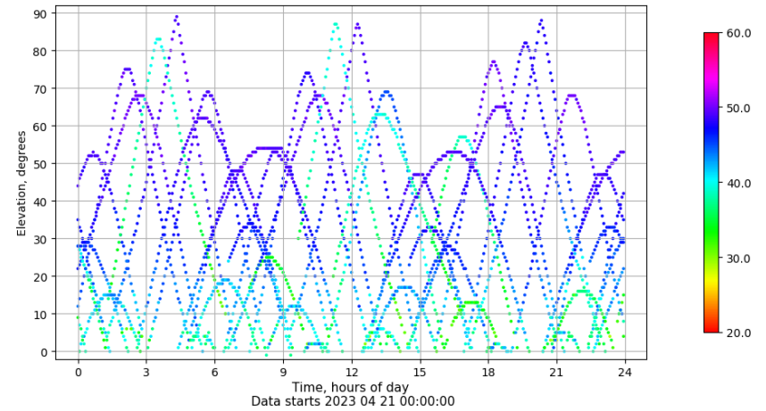
Time-elevation plot for station CAAL. Signal to Noise S1C Data file CAAL00ESP_R_2023111.xtr
