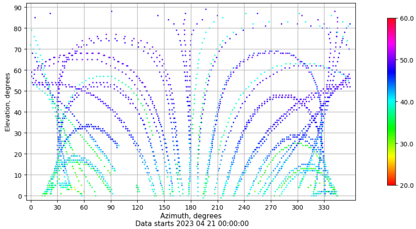
Azimuth-elevation plot for station CAAL. Signal to Noise S1C Data file CAAL00ESP_R_2023111.xtr
