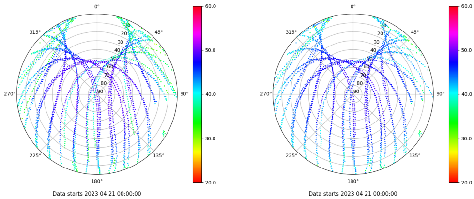
Skyplot for station CAAL. Signal to Noise S1C Data file CAAL00ESP_R_2023111.xtr Skyplot for station CAAL. Signal to Noise S2P Data file CAAL00ESP_R_2023111.xtr
