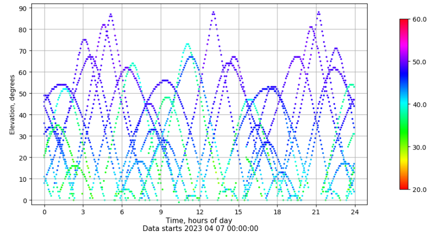
Time-elevation plot for station CAAL. Signal to Noise S1C Data file CAAL00ESP_R_2023097.xtr
