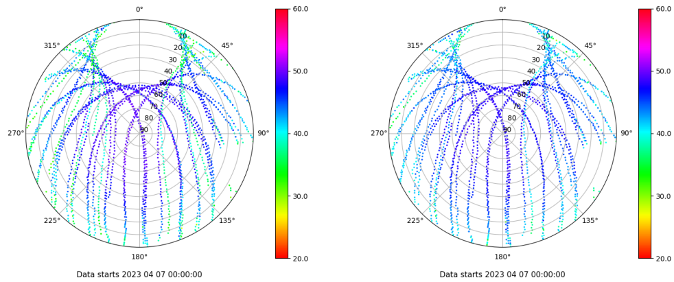
Skyplot for station CAAL. Signal to Noise S1C Data file CAAL00ESP_R_2023097.xtr Skyplot for station CAAL. Signal to Noise S2P Data file CAAL00ESP_R_2023097.xtr
