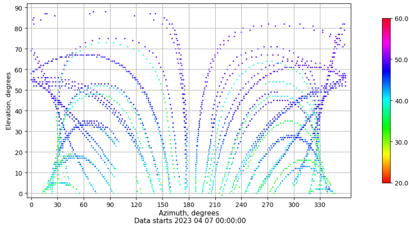
Azimuth-elevation plot for station CAAL. Signal to Noise S1C Data file CAAL00ESP_R_2023097.xtr
