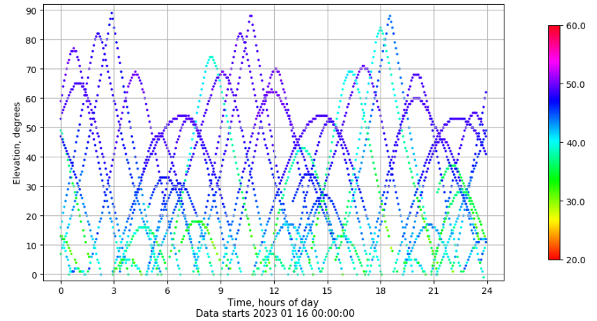
Time-elevation plot for station CAAL. Signal to Noise S1C Data file CAAL00ESP_R_2023016.xtr
