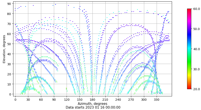
Azimuth-elevation plot for station CAAL. Signal to Noise S1C Data file CAAL00ESP_R_2023016.xtr
