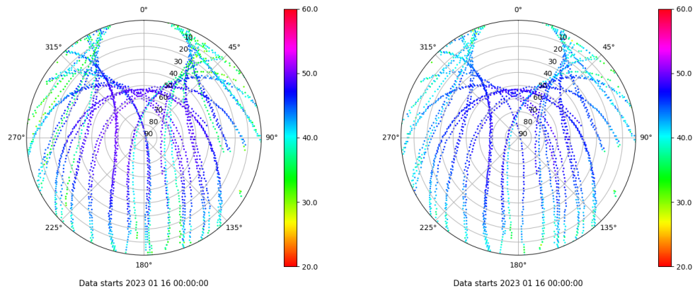
Skyplot for station CAAL. Signal to Noise S1C Data file CAAL00ESP_R_2023016.xtr Skyplot for station CAAL. Signal to Noise S2P Data file CAAL00ESP_R_2023016.xtr
