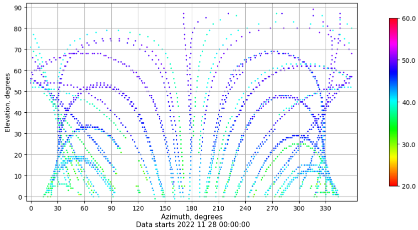
Azimuth-elevation plot for station CAAL. Signal to Noise S1C Data file CAAL00ESP_R_2022332.xtr
