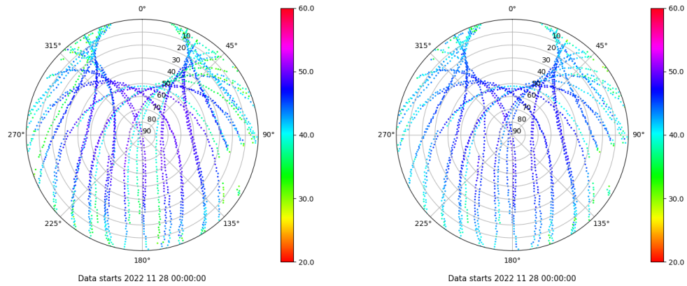
Skyplot for station CAAL. Signal to Noise S1C Data file CAAL00ESP_R_2022332.xtr Skyplot for station CAAL. Signal to Noise S2P Data file CAAL00ESP_R_2022332.xtr
