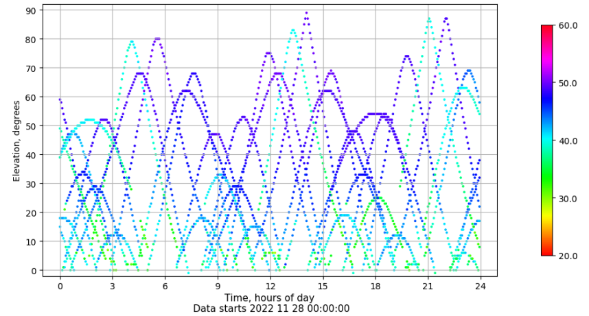
Time-elevation plot for station CAAL. Signal to Noise S1C Data file CAAL00ESP_R_2022332.xtr
