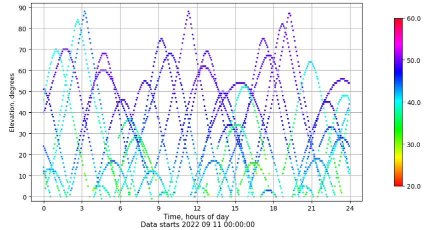
Time-elevation plot for station CAAL. Signal to Noise S1C Data file CAAL00ESP_R_2022254.xtr
