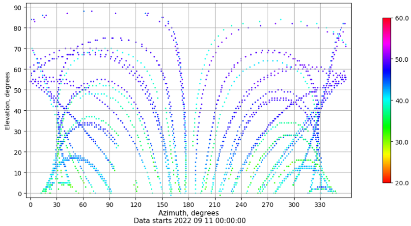
Azimuth-elevation plot for station CAAL. Signal to Noise S1C Data file CAAL00ESP_R_2022254.xtr
