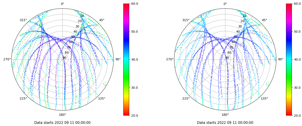
Skyplot for station CAAL. Signal to Noise S1C Data file CAAL00ESP_R_2022254.xtr Skyplot for station CAAL. Signal to Noise S2P Data file CAAL00ESP_R_2022254.xtr
