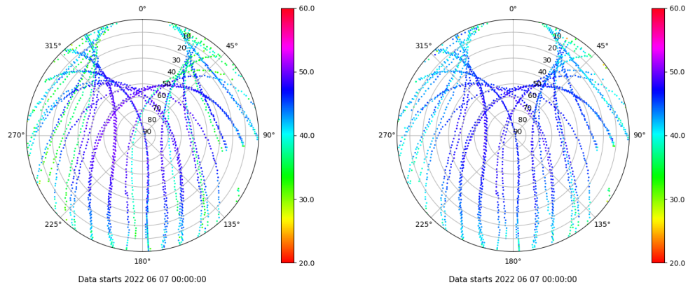
Skyplot for station CAAL. Signal to Noise S1C Data file CAAL00ESP_R_2022158.xtr Skyplot for station CAAL. Signal to Noise S2P Data file CAAL00ESP_R_2022158.xtr
