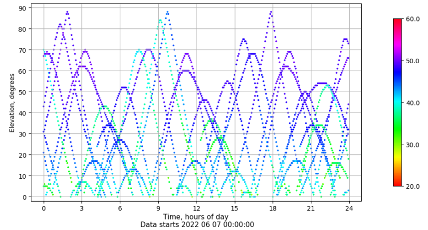
Time-elevation plot for station CAAL. Signal to Noise S1C Data file CAAL00ESP_R_2022158.xtr
