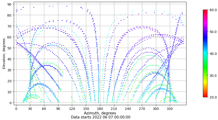
Azimuth-elevation plot for station CAAL. Signal to Noise S1C Data file CAAL00ESP_R_2022158.xtr
