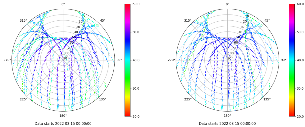
Skyplot for station CAAL. Signal to Noise S1C Data file CAAL00ESP_R_2022074.xtr Skyplot for station CAAL. Signal to Noise S2P Data file CAAL00ESP_R_2022074.xtr
