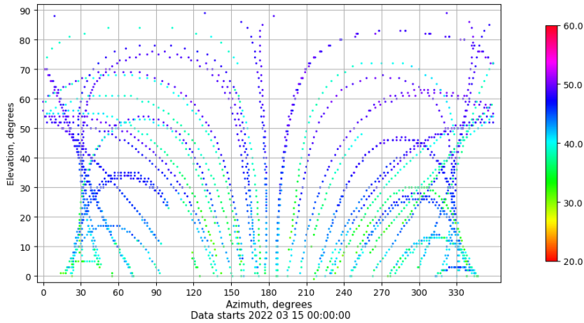
Azimuth-elevation plot for station CAAL. Signal to Noise S1C Data file CAAL00ESP_R_2022074.xtr
