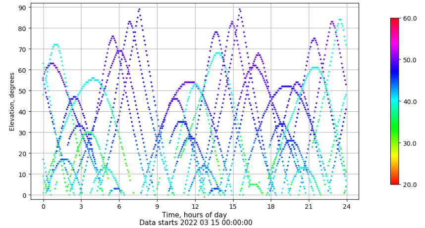
Time-elevation plot for station CAAL. Signal to Noise S1C Data file CAAL00ESP_R_2022074.xtr
