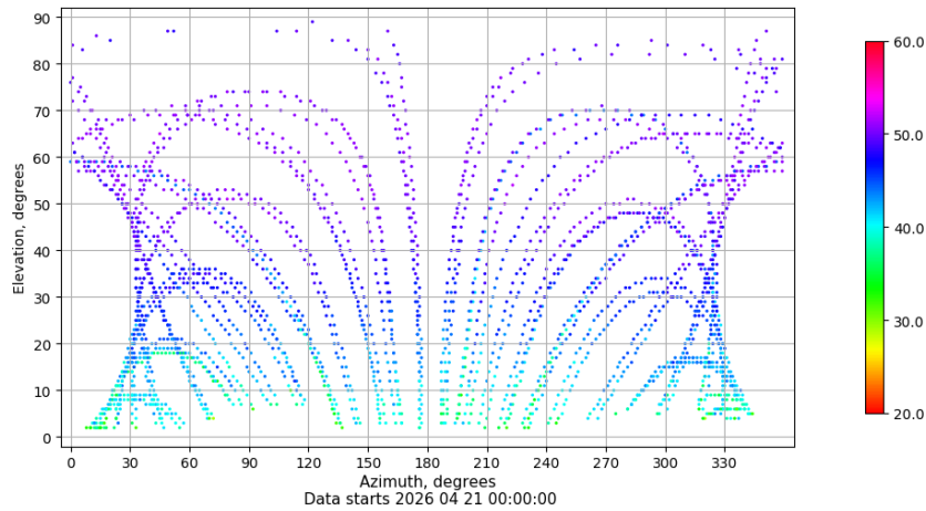
Azimuth-elevation plot for station BUIT. Signal to Noise S1C Data file BUIT00ESP_R_2026111.xtr
