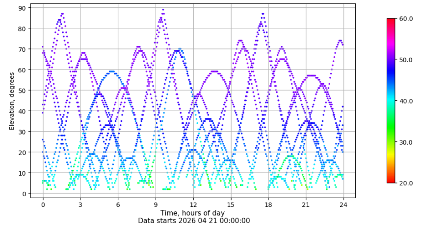
Time-elevation plot for station BUIT. Signal to Noise S1C Data file BUIT00ESP_R_2026111.xtr
