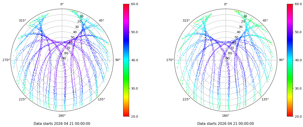
Skyplot for station BUIT. Signal to Noise S1C Data file BUIT00ESP_R_2026111.xtr Skyplot for station BUIT. Signal to Noise S2C Data file BUIT00ESP_R_2026111.xtr
