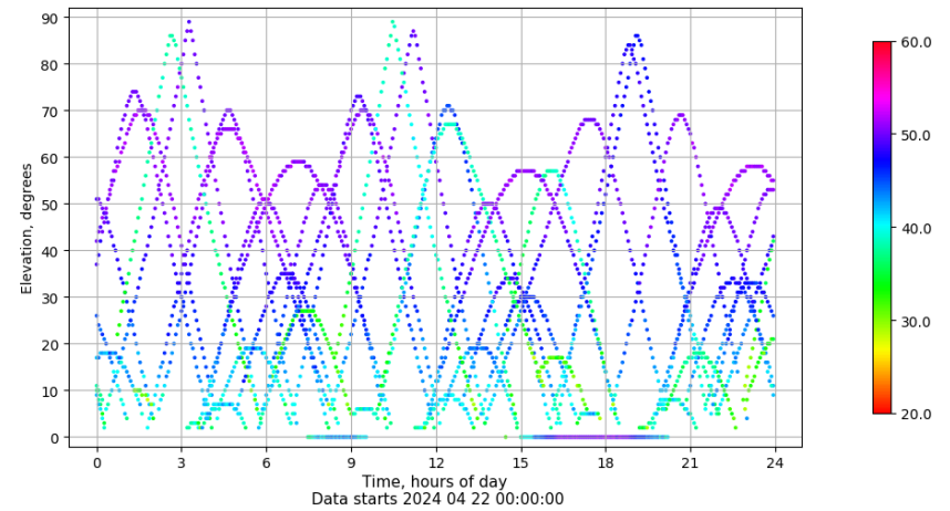
Time-elevation plot for station BUIT. Signal to Noise S1C Data file BUIT00ESP_R_2024113.xtr
