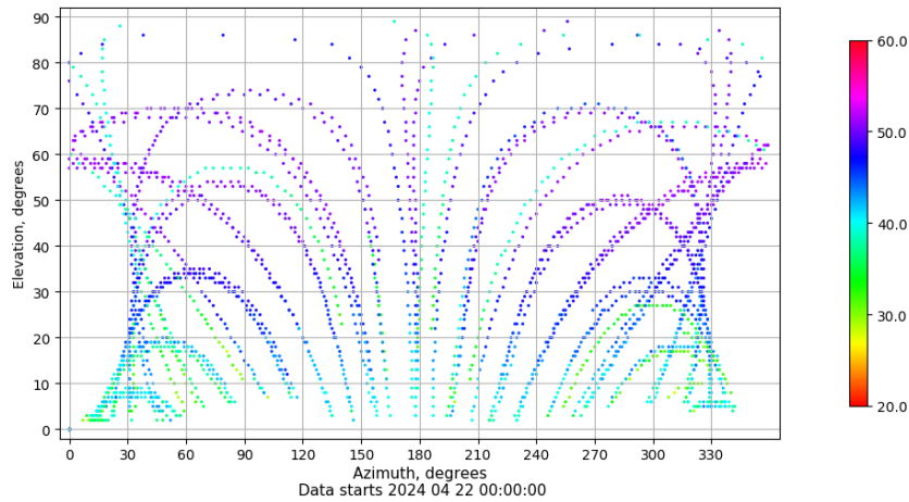
Azimuth-elevation plot for station BUIT. Signal to Noise S1C Data file BUIT00ESP_R_2024113.xtr
