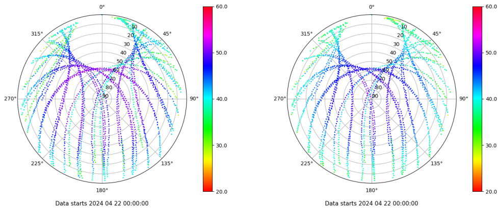
Skyplot for station BUIT. Signal to Noise S1C Data file BUIT00ESP_R_2024113.xtr Skyplot for station BUIT. Signal to Noise S2C Data file BUIT00ESP_R_2024113.xtr
