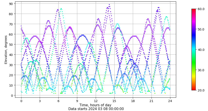
Time-elevation plot for station BUIT. Signal to Noise S1C Data file BUIT00ESP_R_2024068.xtr
