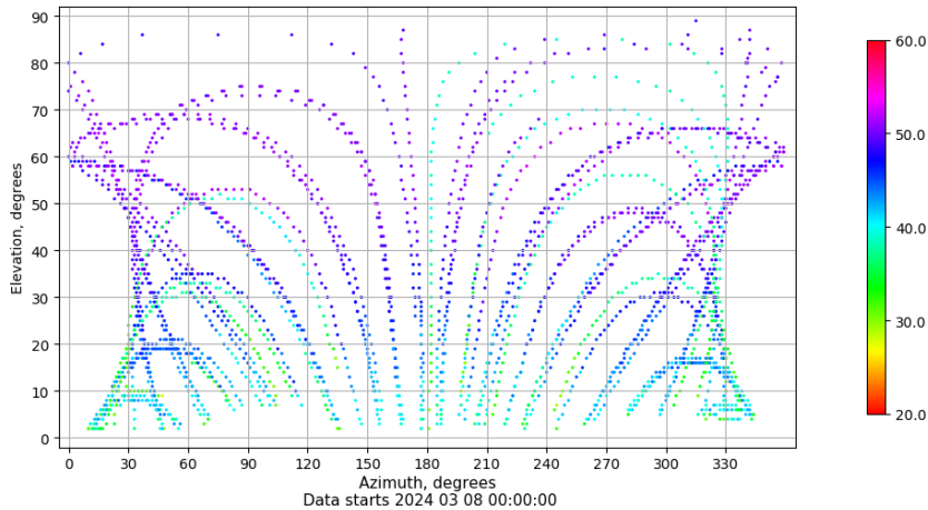
Azimuth-elevation plot for station BUIT. Signal to Noise S1C Data file BUIT00ESP_R_2024068.xtr
