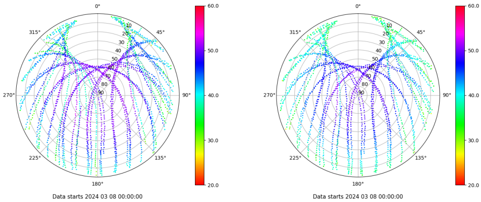
Skyplot for station BUIT. Signal to Noise S1C Data file BUIT00ESP_R_2024068.xtr Skyplot for station BUIT. Signal to Noise S2C Data file BUIT00ESP_R_2024068.xtr
