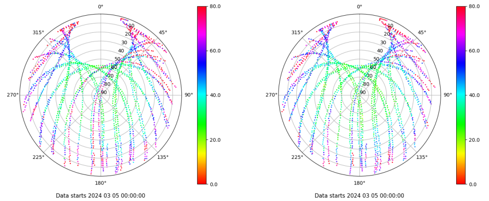
Skyplot for station BUIT. Parameter M1C Data file BUIT00ESP_R_2024065.xtr Skyplot for station BUIT. Parameter M2C Data file BUIT00ESP_R_2024065.xtr
