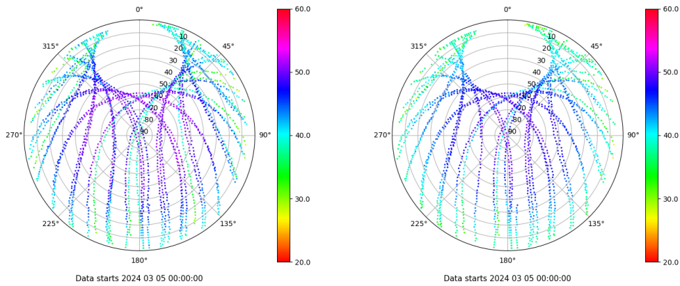
Skyplot for station BUIT. Signal to Noise S1C Data file BUIT00ESP_R_2024065.xtr Skyplot for station BUIT. Signal to Noise S2C Data file BUIT00ESP_R_2024065.xtr
