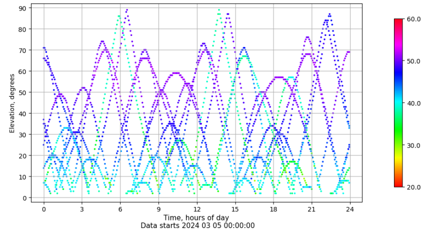
Time-elevation plot for station BUIT. Signal to Noise S1C Data file BUIT00ESP_R_2024065.xtr
