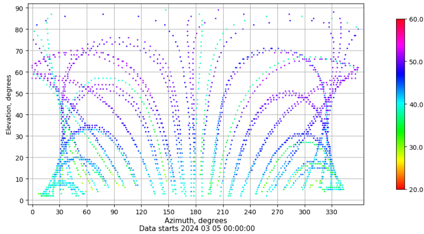
Azimuth-elevation plot for station BUIT. Signal to Noise S1C Data file BUIT00ESP_R_2024065.xtr
