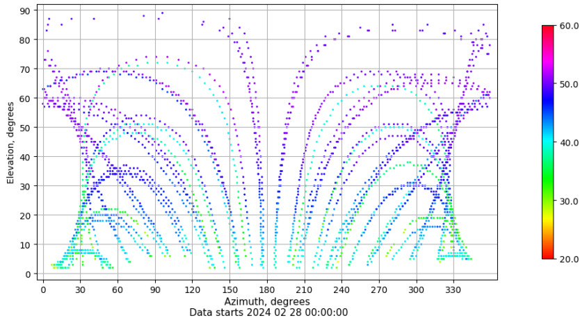
Azimuth-elevation plot for station BUIT. Signal to Noise S1C Data file BUIT00ESP_R_2024059.xtr
