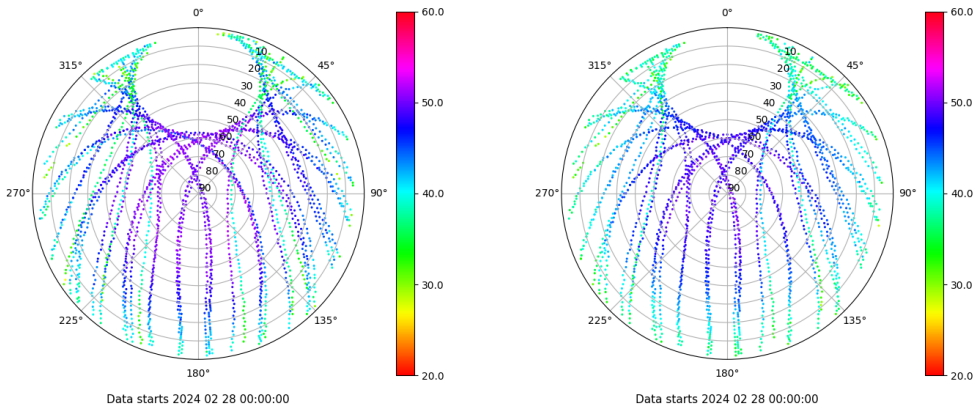
Skyplot for station BUIT. Signal to Noise S1C Data file BUIT00ESP_R_2024059.xtr Skyplot for station BUIT. Signal to Noise S2C Data file BUIT00ESP_R_2024059.xtr
