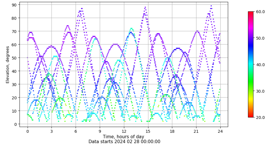
Time-elevation plot for station BUIT. Signal to Noise S1C Data file BUIT00ESP_R_2024059.xtr
