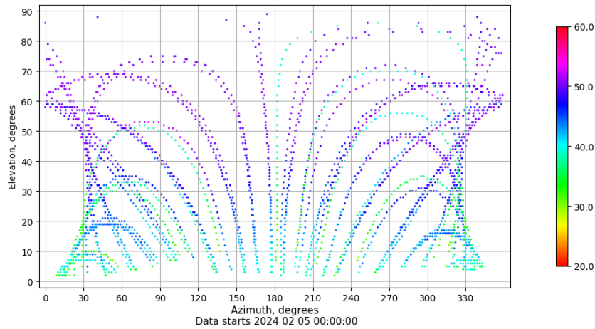
Azimuth-elevation plot for station BUIT. Signal to Noise S1C Data file BUIT00ESP_R_2024036.xtr
