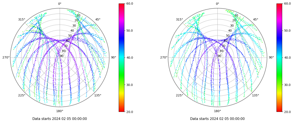
Skyplot for station BUIT. Signal to Noise S1C Data file BUIT00ESP_R_2024036.xtr Skyplot for station BUIT. Signal to Noise S2C Data file BUIT00ESP_R_2024036.xtr
