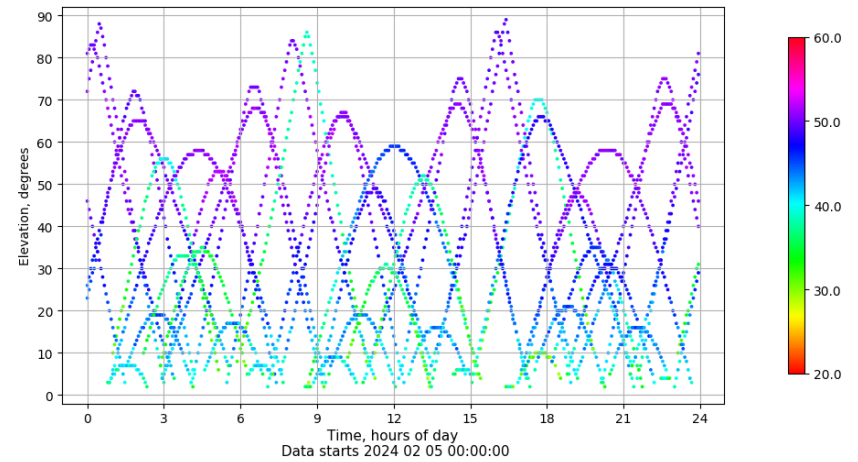
Time-elevation plot for station BUIT. Signal to Noise S1C Data file BUIT00ESP_R_2024036.xtr
