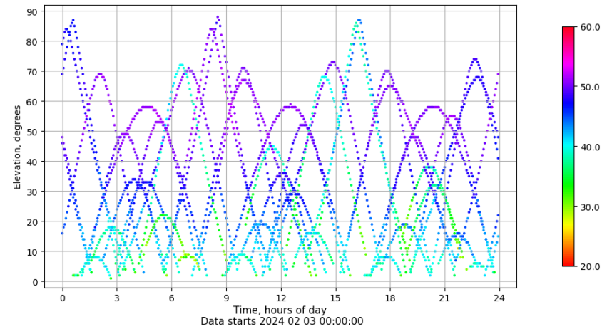
Time-elevation plot for station BUIT. Signal to Noise S1C Data file BUIT00ESP_R_2024034.xtr
