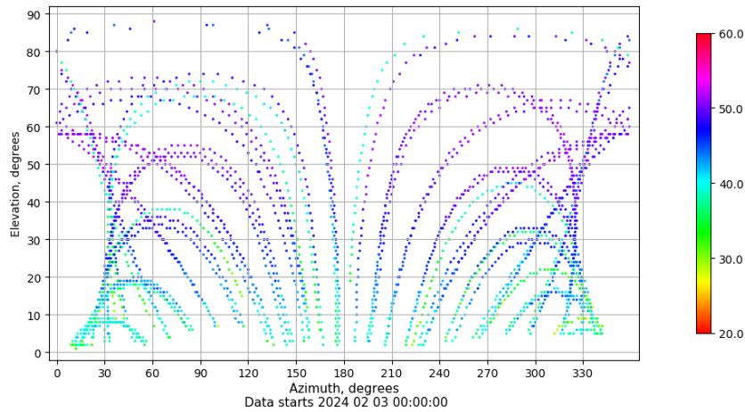
Azimuth-elevation plot for station BUIT. Signal to Noise S1C Data file BUIT00ESP_R_2024034.xtr
