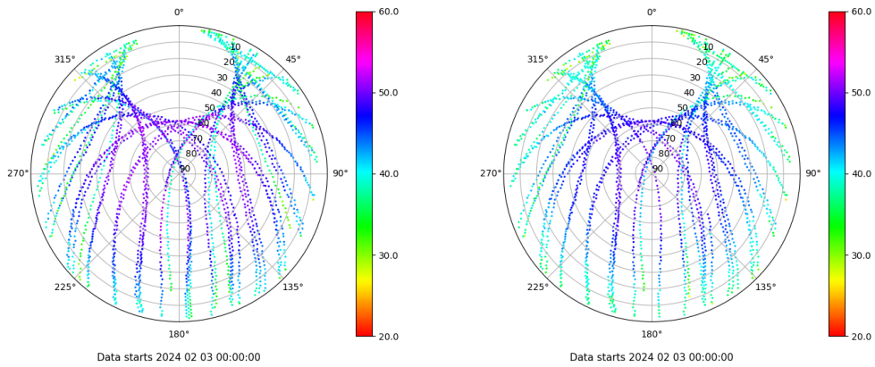
Skyplot for station BUIT. Signal to Noise S1C Data file BUIT00ESP_R_2024034.xtr Skyplot for station BUIT. Signal to Noise S2C Data file BUIT00ESP_R_2024034.xtr
