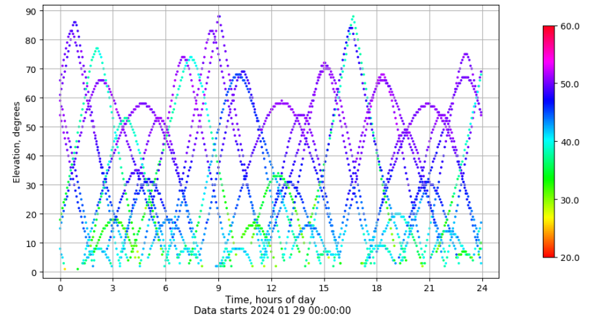
Time-elevation plot for station BUIT. Signal to Noise S1C Data file BUIT00ESP_R_2024029.xtr
