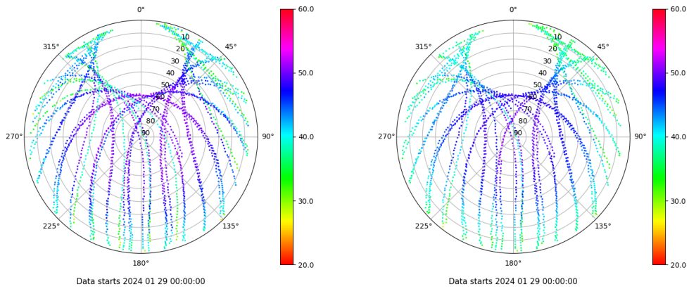
Skyplot for station BUIT. Signal to Noise S1C Data file BUIT00ESP_R_2024029.xtr Skyplot for station BUIT. Signal to Noise S2C Data file BUIT00ESP_R_2024029.xtr
