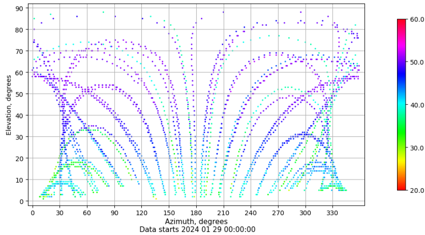
Azimuth-elevation plot for station BUIT. Signal to Noise S1C Data file BUIT00ESP_R_2024029.xtr
