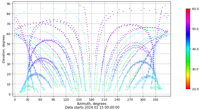
Azimuth-elevation plot for station BUIT. Signal to Noise S1C Data file BUIT00ESP_R_2024015.xtr
