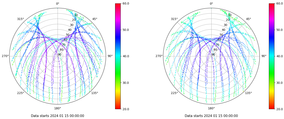
Skyplot for station BUIT. Signal to Noise S1C Data file BUIT00ESP_R_2024015.xtr Skyplot for station BUIT. Signal to Noise S2C Data file BUIT00ESP_R_2024015.xtr
