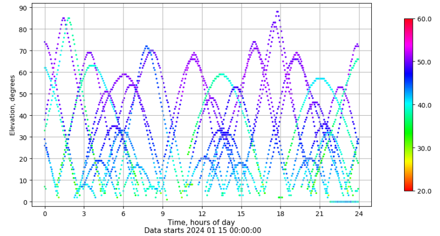
Time-elevation plot for station BUIT. Signal to Noise S1C Data file BUIT00ESP_R_2024015.xtr
