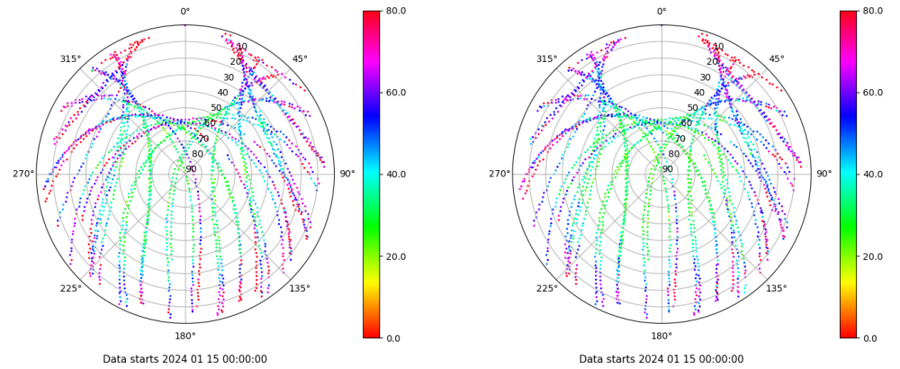
Skyplot for station BUIT. Parameter M1C Data file BUIT00ESP_R_2024015.xtr Skyplot for station BUIT. Parameter M2C Data file BUIT00ESP_R_2024015.xtr
