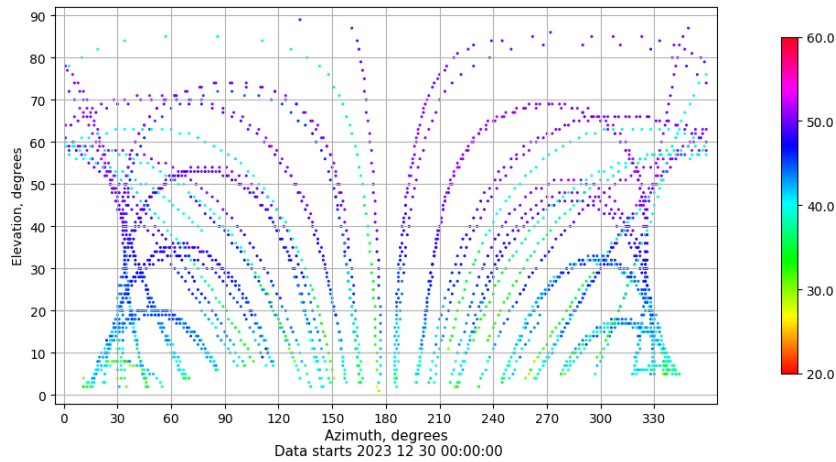
Azimuth-elevation plot for station BUIT. Signal to Noise S1C Data file BUIT00ESP_R_2023364.xtr
