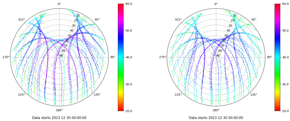
Skyplot for station BUIT. Signal to Noise S1C Data file BUIT00ESP_R_2023364.xtr Skyplot for station BUIT. Signal to Noise S2C Data file BUIT00ESP_R_2023364.xtr
