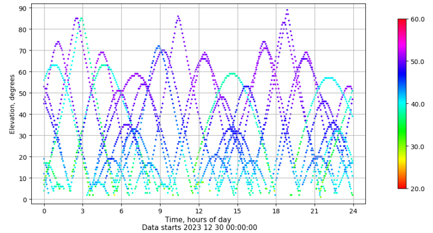
Time-elevation plot for station BUIT. Signal to Noise S1C Data file BUIT00ESP_R_2023364.xtr
