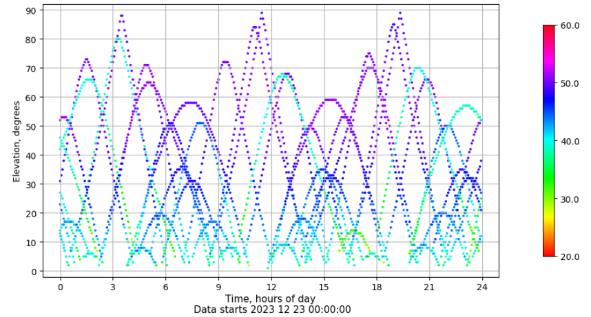
Time-elevation plot for station BUIT. Signal to Noise S1C Data file BUIT00ESP_R_2023357.xtr
