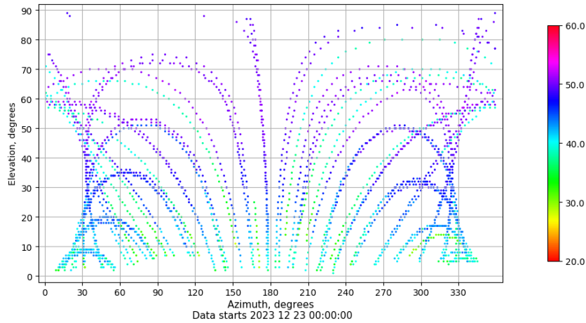
Azimuth-elevation plot for station BUIT. Signal to Noise S1C Data file BUIT00ESP_R_2023357.xtr
