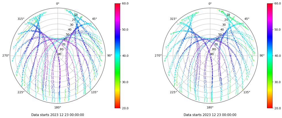
Skyplot for station BUIT. Signal to Noise S1C Data file BUIT00ESP_R_2023357.xtr Skyplot for station BUIT. Signal to Noise S2C Data file BUIT00ESP_R_2023357.xtr
