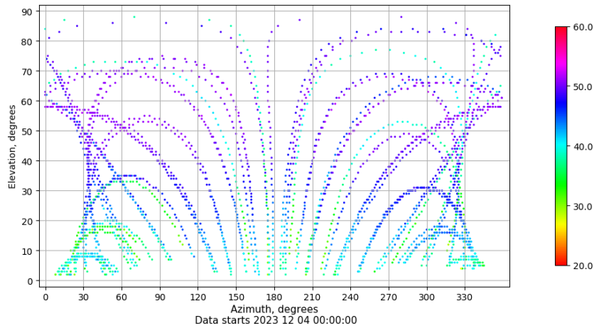
Azimuth-elevation plot for station BUIT. Signal to Noise S1C Data file BUIT00ESP_R_2023338.xtr
