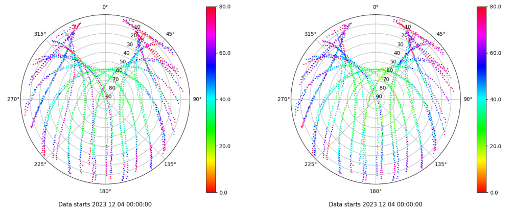
Skyplot for station BUIT. Parameter M1C Data file BUIT00ESP_R_2023338.xtr Skyplot for station BUIT. Parameter M2C Data file BUIT00ESP_R_2023338.xtr
