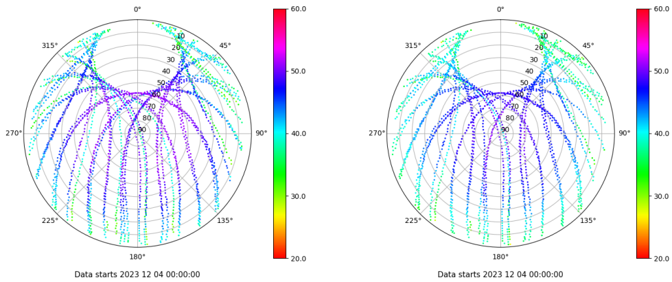
Skyplot for station BUIT. Signal to Noise S1C Data file BUIT00ESP_R_2023338.xtr Skyplot for station BUIT. Signal to Noise S2C Data file BUIT00ESP_R_2023338.xtr
