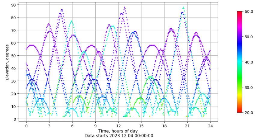
Time-elevation plot for station BUIT. Signal to Noise S1C Data file BUIT00ESP_R_2023338.xtr
