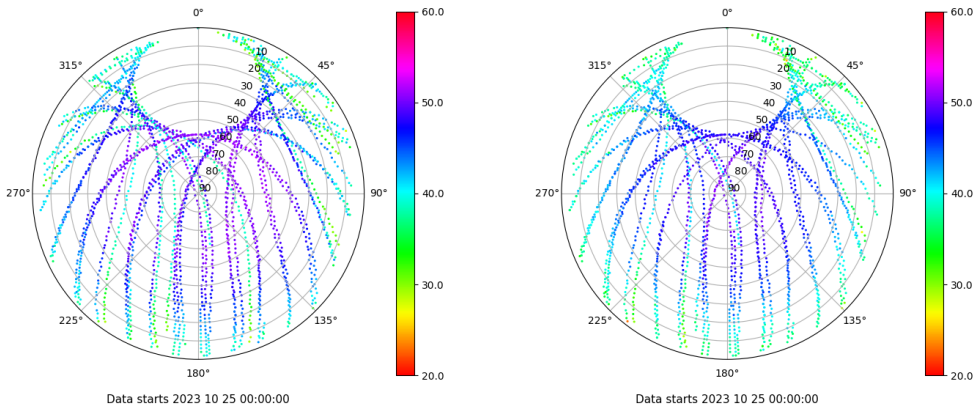
Skyplot for station BUIT. Signal to Noise S1C Data file BUIT00ESP_R_2023298.xtr Skyplot for station BUIT. Signal to Noise S2C Data file BUIT00ESP_R_2023298.xtr
