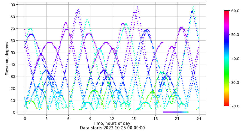
Time-elevation plot for station BUIT. Signal to Noise S1C Data file BUIT00ESP_R_2023298.xtr
