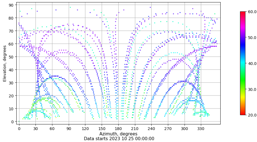
Azimuth-elevation plot for station BUIT. Signal to Noise S1C Data file BUIT00ESP_R_2023298.xtr
