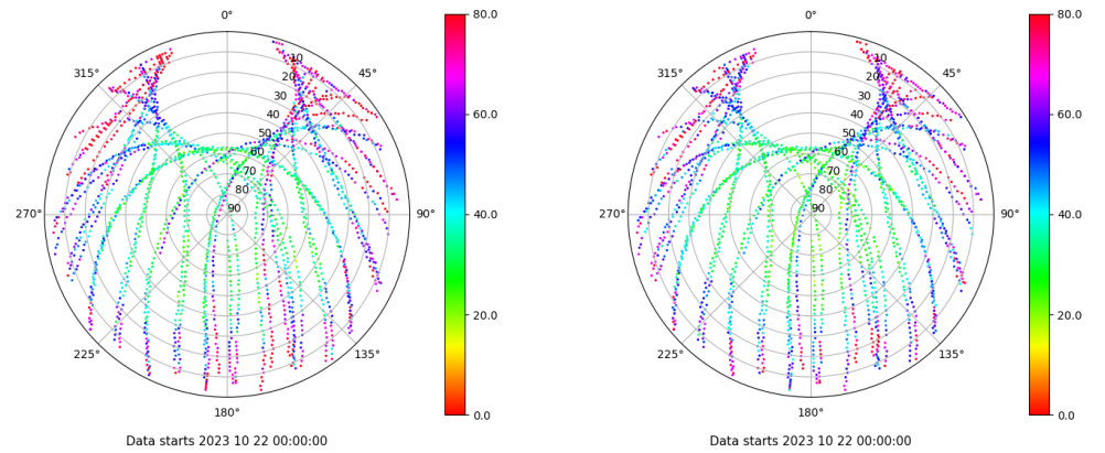
Skyplot for station BUIT. Parameter M1C Data file BUIT00ESP_R_2023295.xtr Skyplot for station BUIT. Parameter M2C Data file BUIT00ESP_R_2023295.xtr
