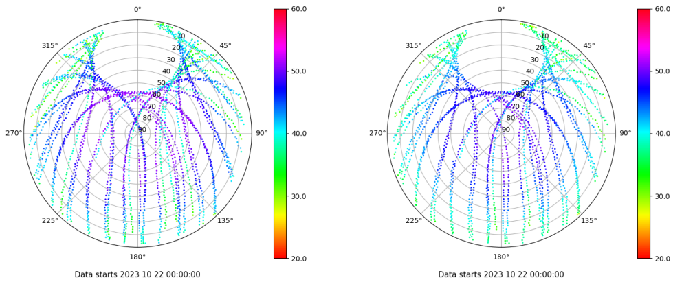
Skyplot for station BUIT. Signal to Noise S1C Data file BUIT00ESP_R_2023295.xtr Skyplot for station BUIT. Signal to Noise S2C Data file BUIT00ESP_R_2023295.xtr
