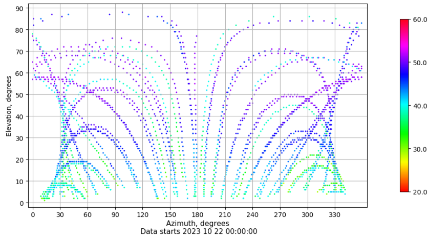
Azimuth-elevation plot for station BUIT. Signal to Noise S1C Data file BUIT00ESP_R_2023295.xtr
