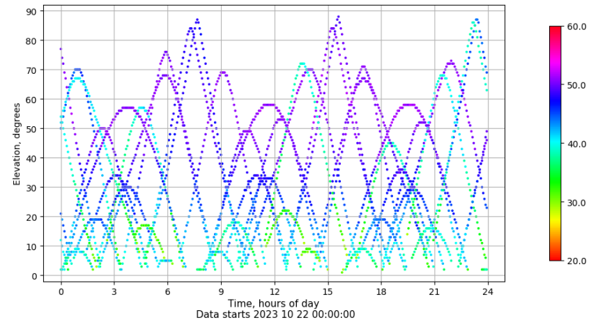
Time-elevation plot for station BUIT. Signal to Noise S1C Data file BUIT00ESP_R_2023295.xtr
