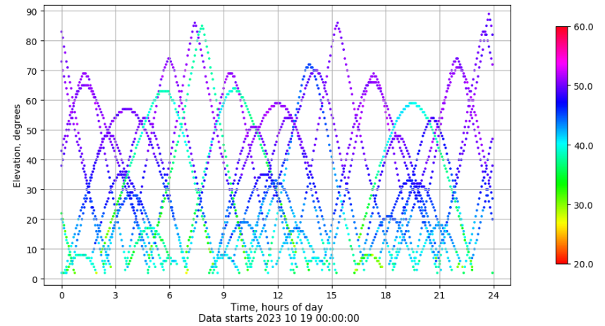
Time-elevation plot for station BUIT. Signal to Noise S1C Data file BUIT00ESP_R_2023292.xtr
