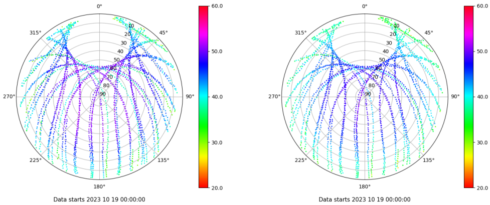
Skyplot for station BUIT. Signal to Noise S1C Data file BUIT00ESP_R_2023292.xtr Skyplot for station BUIT. Signal to Noise S2C Data file BUIT00ESP_R_2023292.xtr
