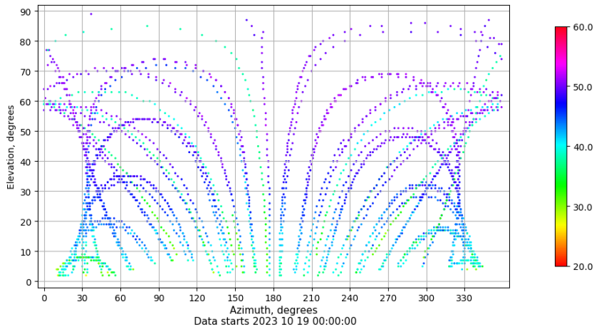
Azimuth-elevation plot for station BUIT. Signal to Noise S1C Data file BUIT00ESP_R_2023292.xtr
