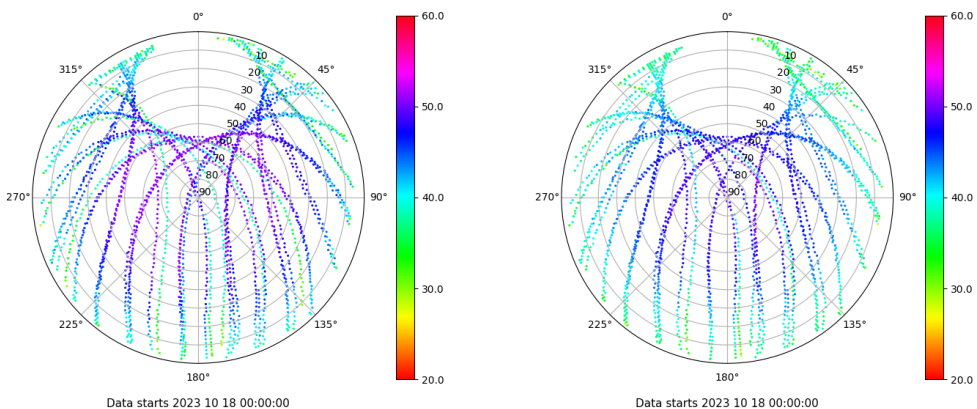
Skyplot for station BUIT. Signal to Noise S1C Data file BUIT00ESP_R_2023291.xtr Skyplot for station BUIT. Signal to Noise S2C Data file BUIT00ESP_R_2023291.xtr
