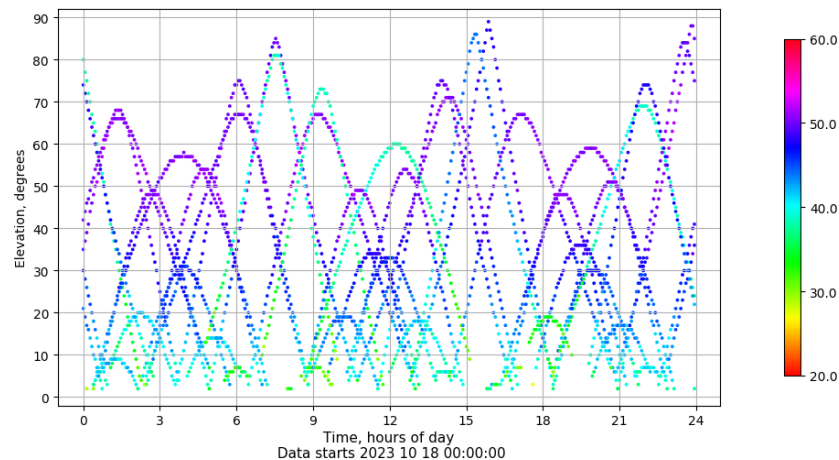
Time-elevation plot for station BUIT. Signal to Noise S1C Data file BUIT00ESP_R_2023291.xtr
