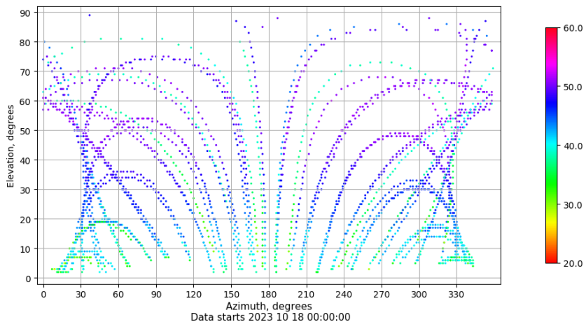
Azimuth-elevation plot for station BUIT. Signal to Noise S1C Data file BUIT00ESP_R_2023291.xtr
