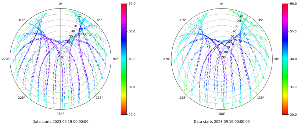
Skyplot for station BUIT. Signal to Noise S1C Data file BUIT00ESP_R_2023262.xtr Skyplot for station BUIT. Signal to Noise S2C Data file BUIT00ESP_R_2023262.xtr
