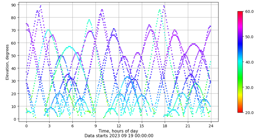
Time-elevation plot for station BUIT. Signal to Noise S1C Data file BUIT00ESP_R_2023262.xtr
