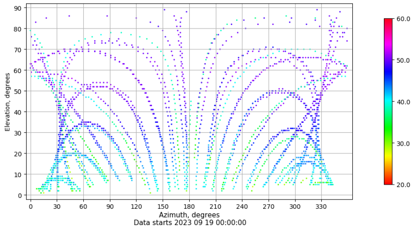
Azimuth-elevation plot for station BUIT. Signal to Noise S1C Data file BUIT00ESP_R_2023262.xtr
