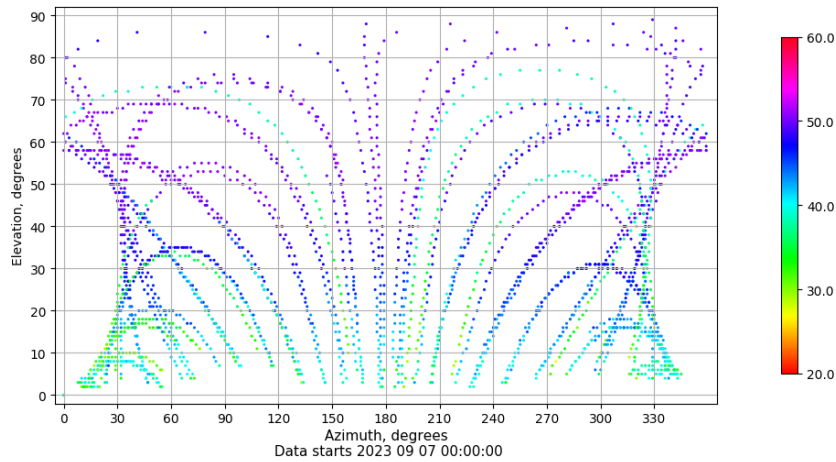
Azimuth-elevation plot for station BUIT. Signal to Noise S1C Data file BUIT00ESP_R_2023250.xtr
