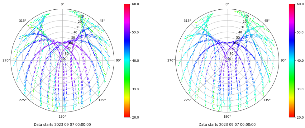
Skyplot for station BUIT. Signal to Noise S1C Data file BUIT00ESP_R_2023250.xtr Skyplot for station BUIT. Signal to Noise S2C Data file BUIT00ESP_R_2023250.xtr
