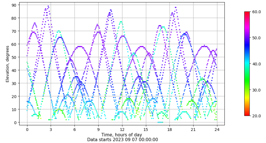
Time-elevation plot for station BUIT. Signal to Noise S1C Data file BUIT00ESP_R_2023250.xtr
