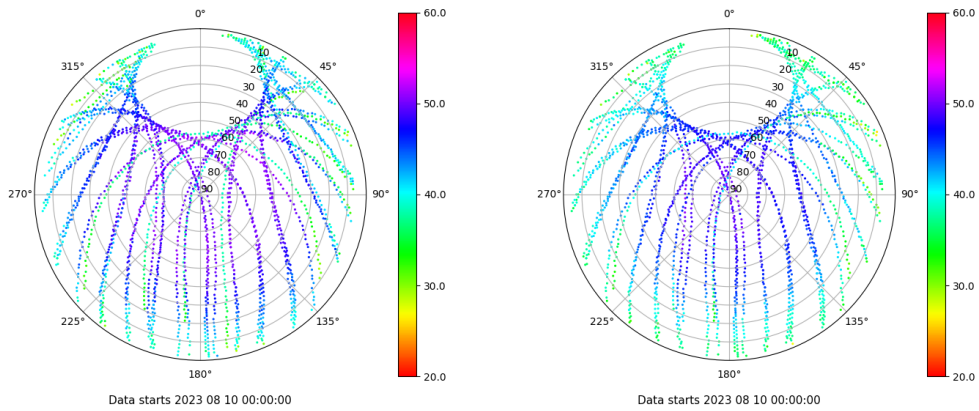
Skyplot for station BUIT. Signal to Noise S1C Data file BUIT00ESP_R_2023222.xtr Skyplot for station BUIT. Signal to Noise S2C Data file BUIT00ESP_R_2023222.xtr
