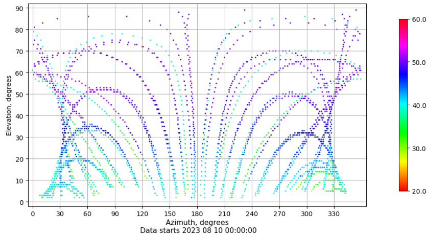
Azimuth-elevation plot for station BUIT. Signal to Noise S1C Data file BUIT00ESP_R_2023222.xtr
