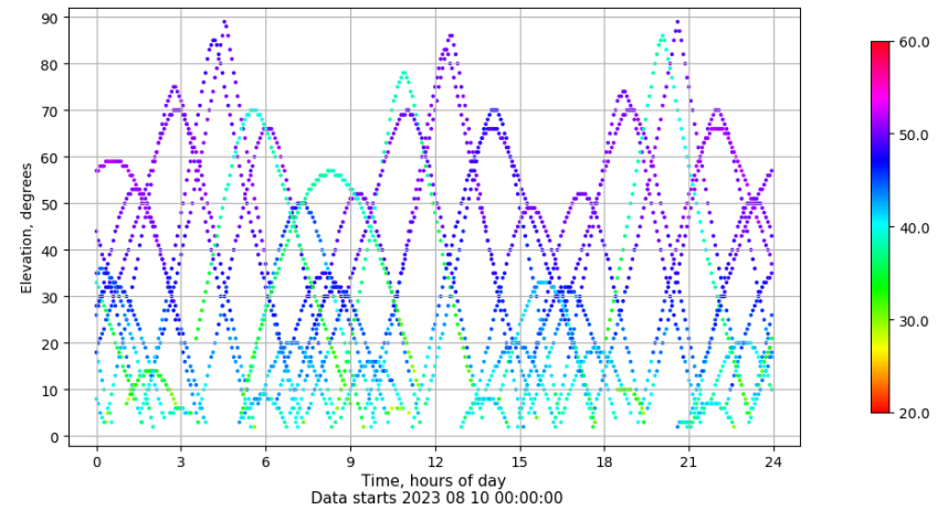
Time-elevation plot for station BUIT. Signal to Noise S1C Data file BUIT00ESP_R_2023222.xtr
