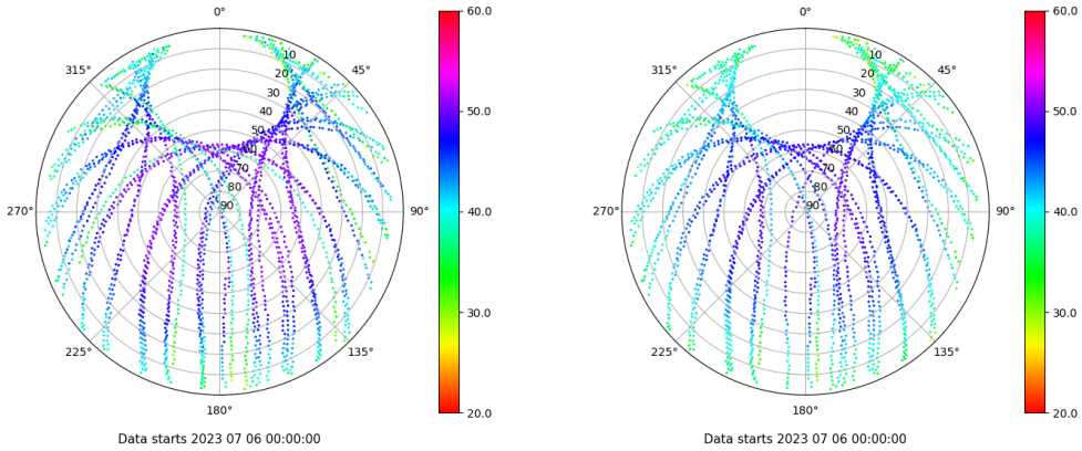
Skyplot for station BUIT. Signal to Noise S1C Data file BUIT00ESP_R_2023187.xtr Skyplot for station BUIT. Signal to Noise S2C Data file BUIT00ESP_R_2023187.xtr
