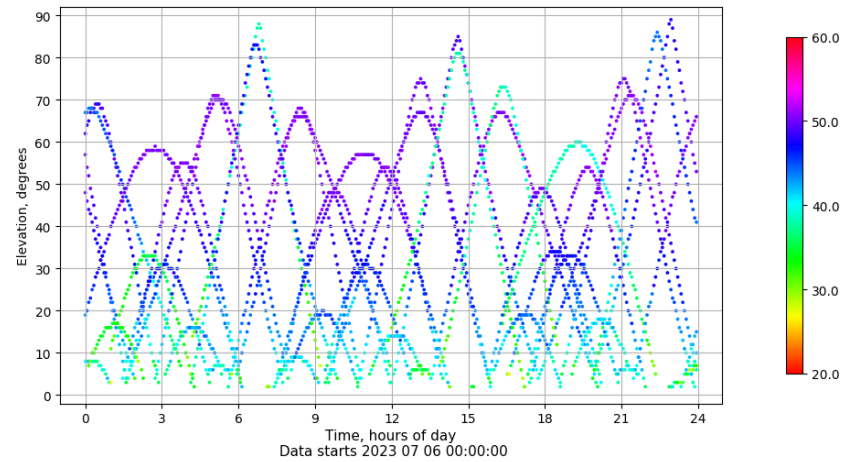
Time-elevation plot for station BUIT. Signal to Noise S1C Data file BUIT00ESP_R_2023187.xtr
