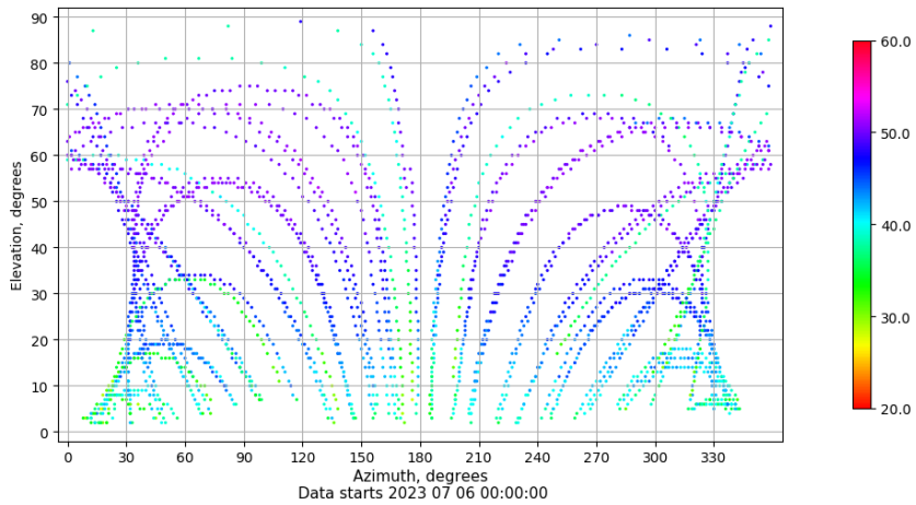
Azimuth-elevation plot for station BUIT. Signal to Noise S1C Data file BUIT00ESP_R_2023187.xtr
